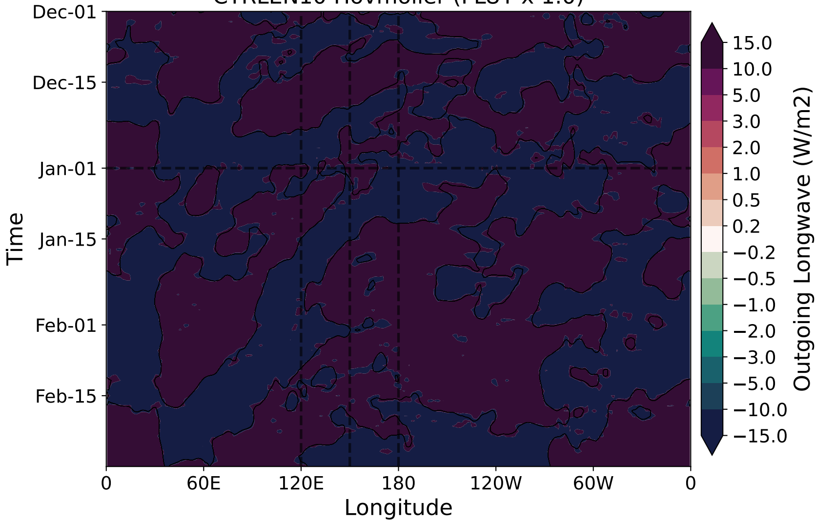
CTRLLEN10 Hovmoller (FLUT x 1.0)
