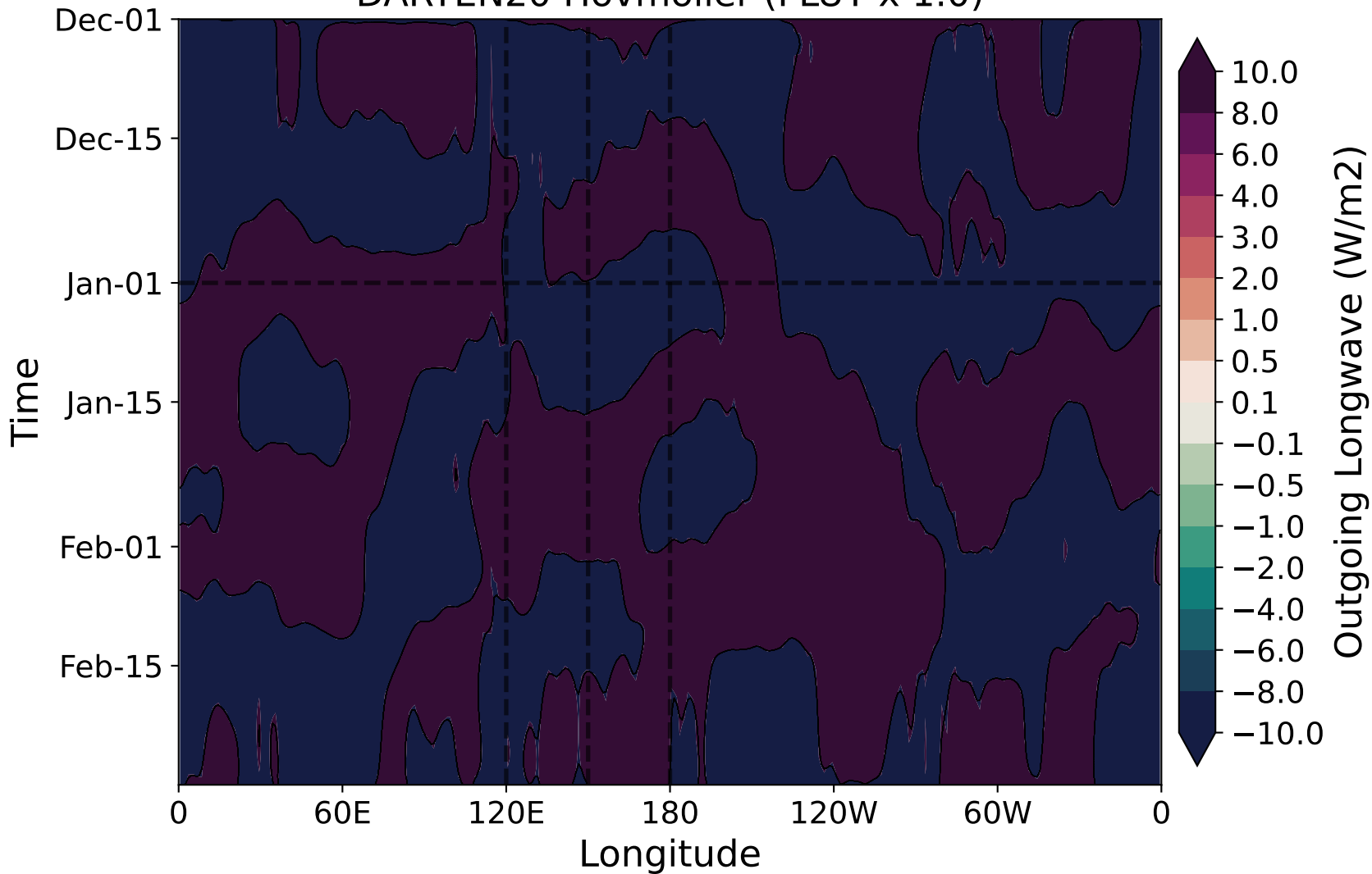
DARTEN20 Hovmoller (FLUT x 1.0)
