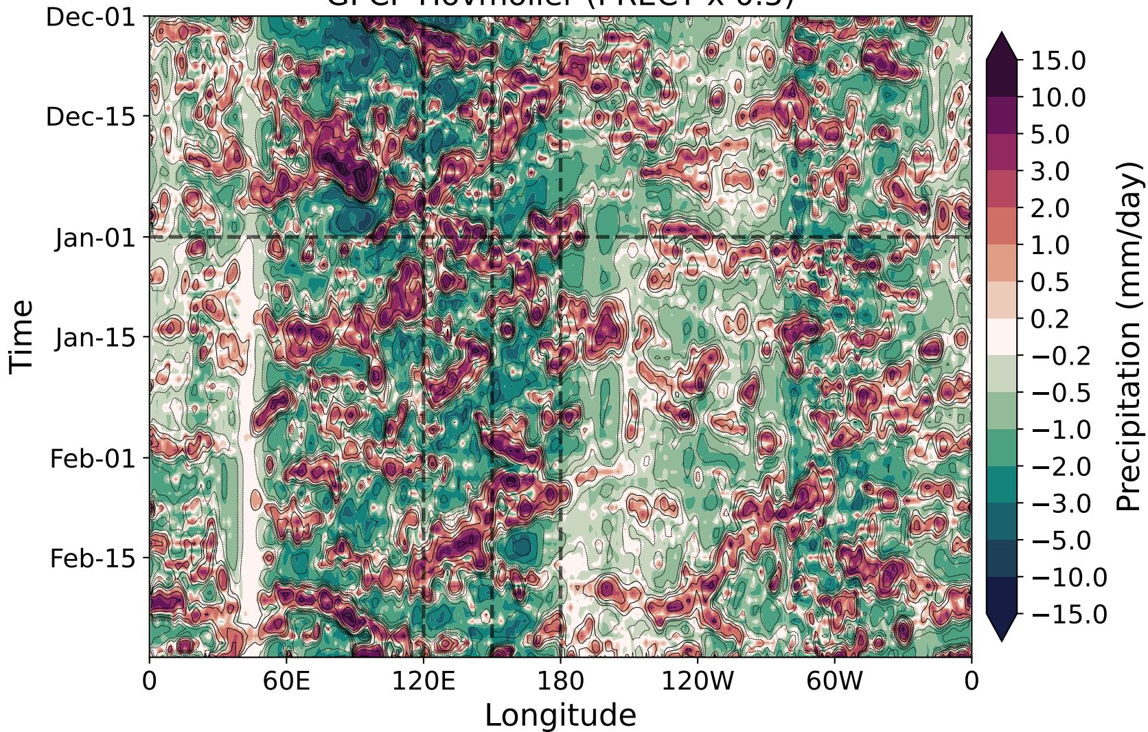
GPCP Hovmoller (PRECT x 0.5)
