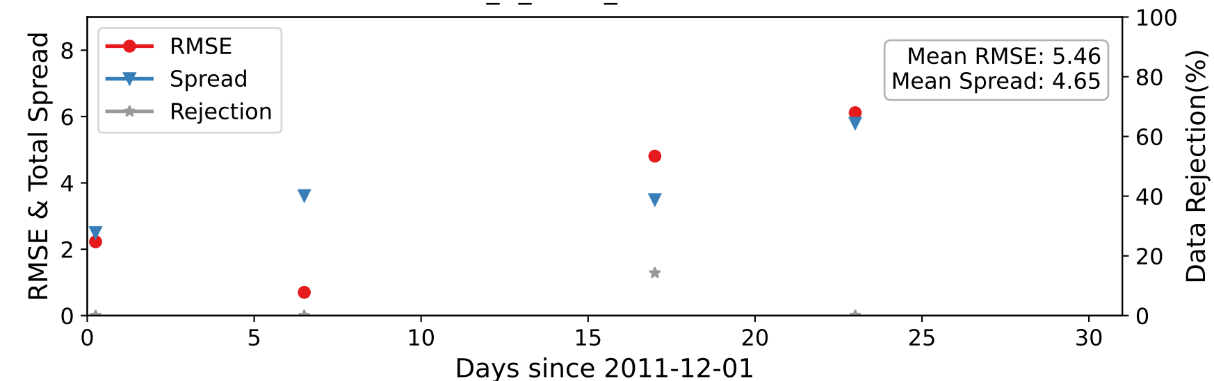
DARTEN10 — ACARS_U_WIND_COMPONENT at 125-175 hPa
