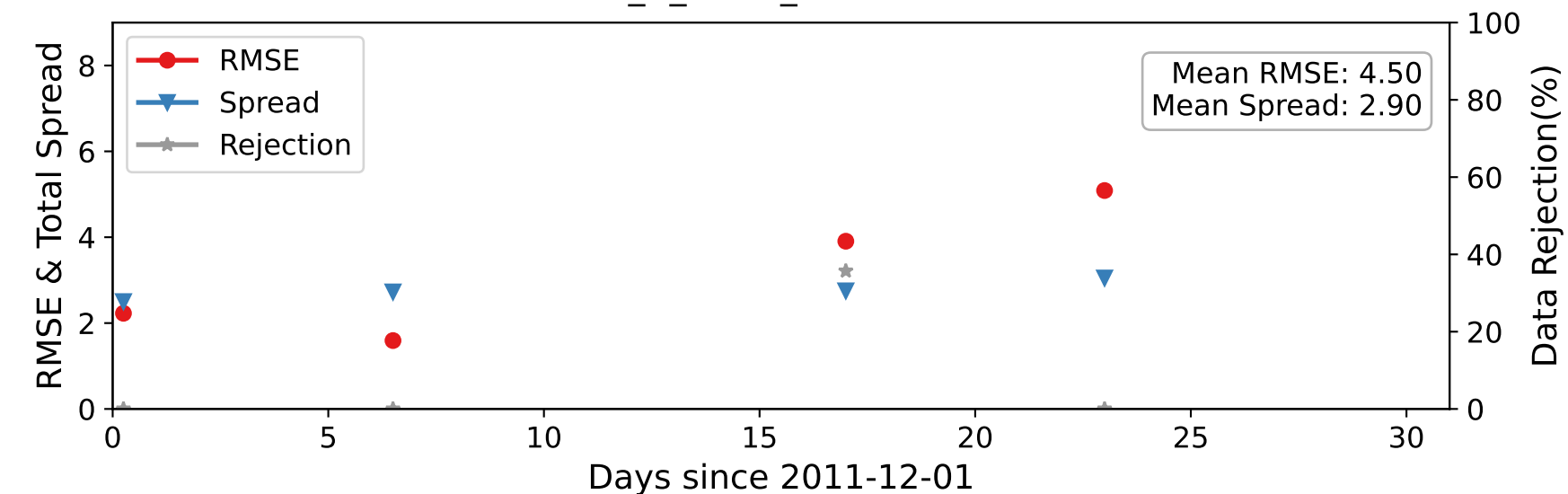
DARTEN40 — ACARS_U_WIND_COMPONENT at 125-175 hPa
