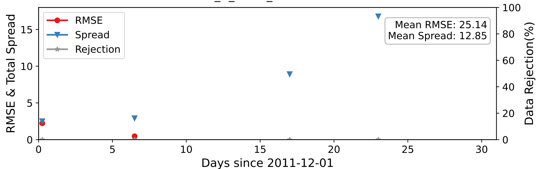
CTRLN10 — ACARS_U_WIND_COMPONENT at 125-175 hPa
