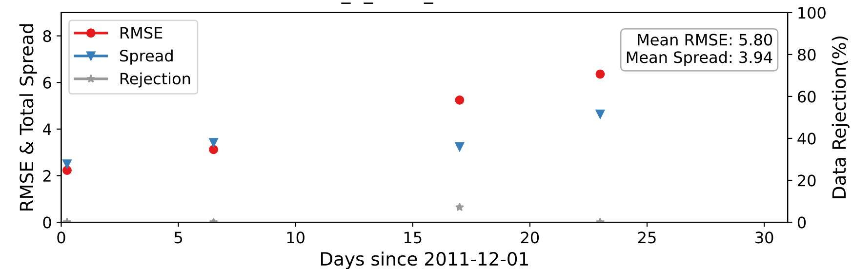
DARTEN20 — ACARS_U_WIND_COMPONENT at 125-175 hPa
