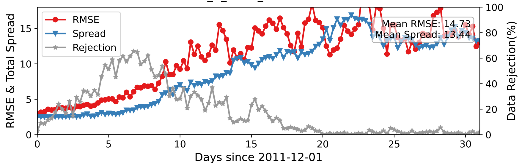
CTRLN10 — ACARS_U_WIND_COMPONENT at 175-225 hPa
