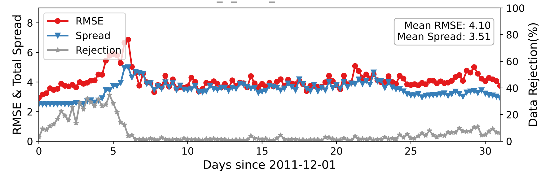
DARTEN20 — ACARS_U_WIND_COMPONENT at 175-225 hPa
