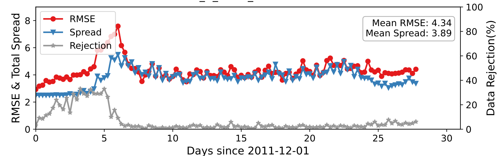
DARTEN10 — ACARS_U_WIND_COMPONENT at 175-225 hPa
