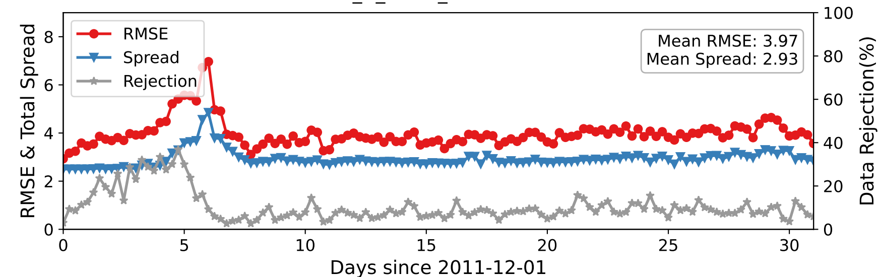
DARTEN40 — ACARS_U_WIND_COMPONENT at 175-225 hPa
