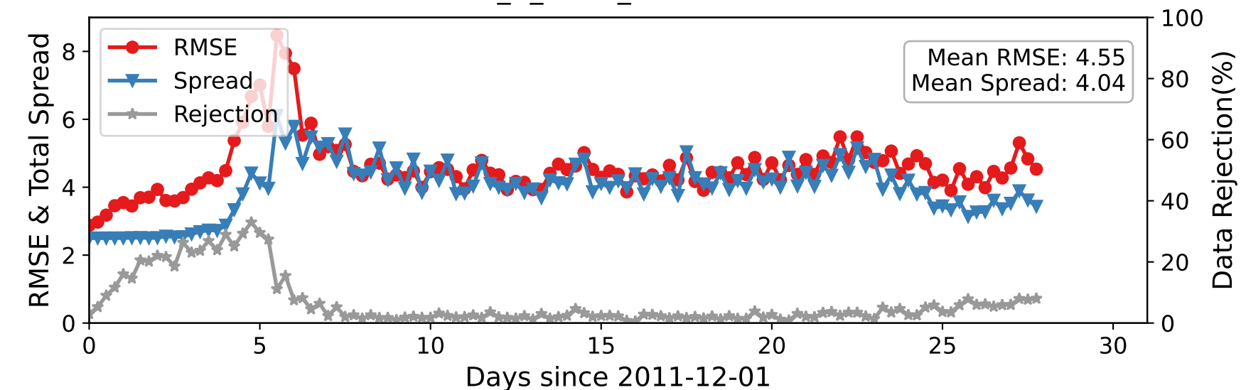
DARTEN10 — ACARS_U_WIND_COMPONENT at 225-275 hPa
