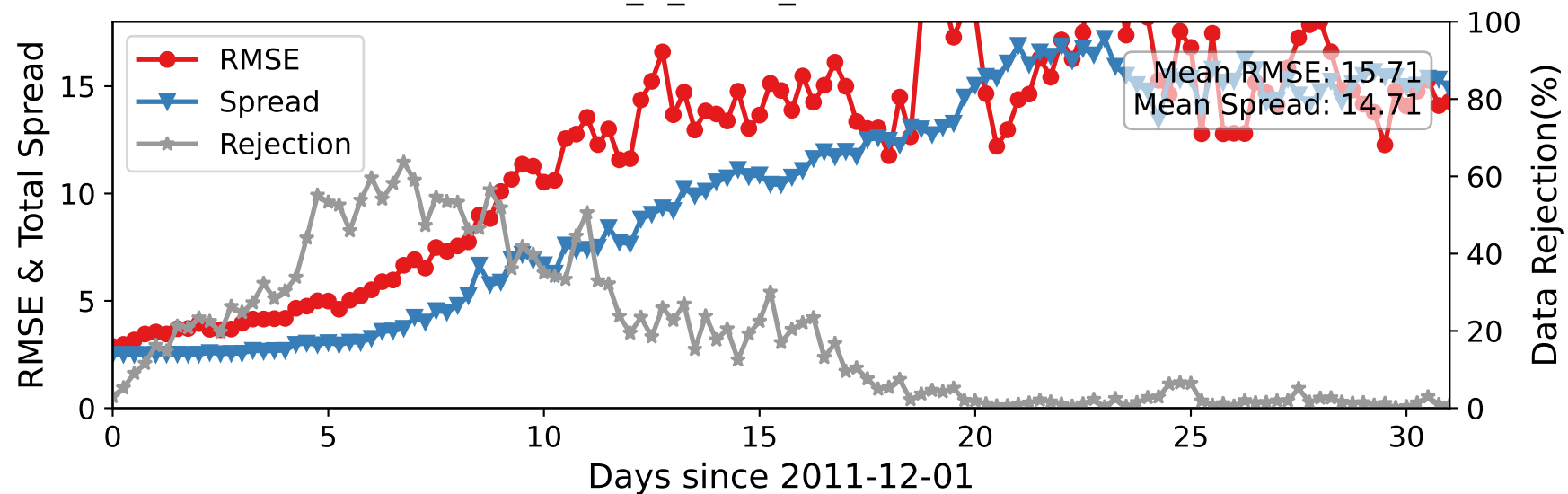
CTRLN10 — ACARS_U_WIND_COMPONENT at 225-275 hPa
