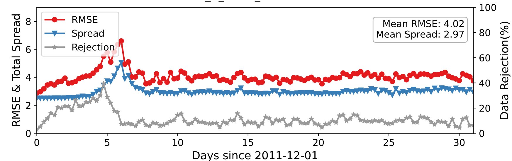
DARTEN40 — ACARS_U_WIND_COMPONENT at 225-275 hPa
