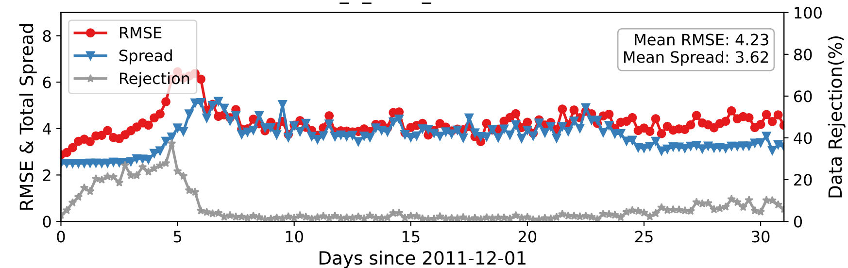
DARTEN20 — ACARS_U_WIND_COMPONENT at 225-275 hPa
