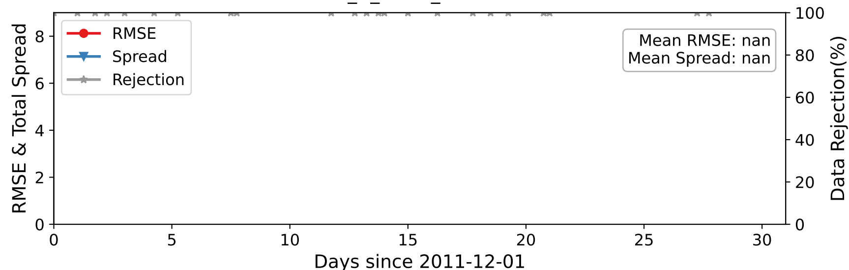
DARTEN20 — ACARS_U_WIND_COMPONENT at 35-75 hPa
