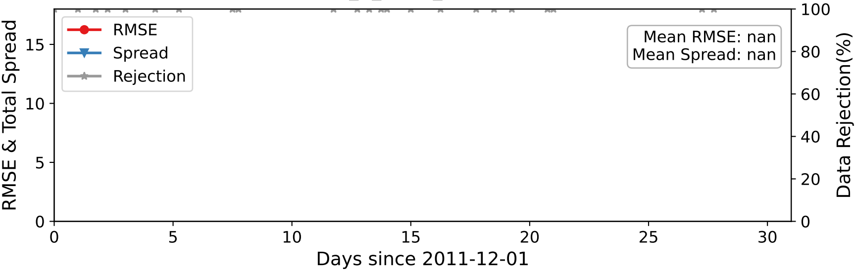
CTRLN10 — ACARS_U_WIND_COMPONENT at 35-75 hPa
