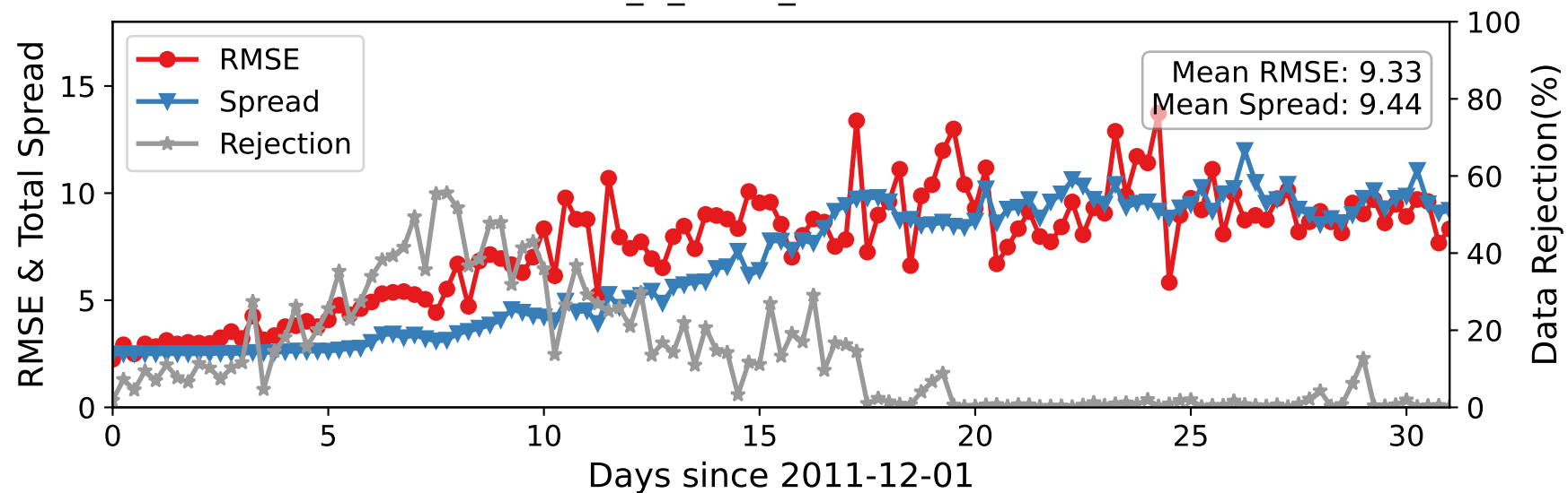
CTRLN10 — ACARS_U_WIND_COMPONENT at 450-600 hPa
