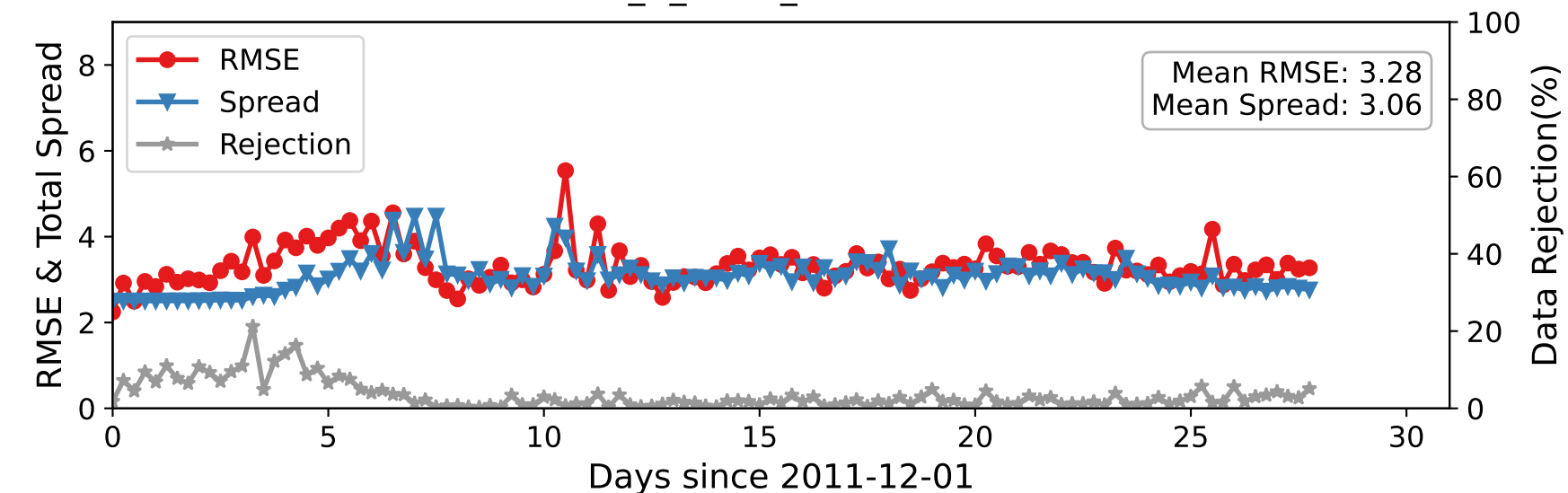
DARTEN10 — ACARS_U_WIND_COMPONENT at 450-600 hPa
