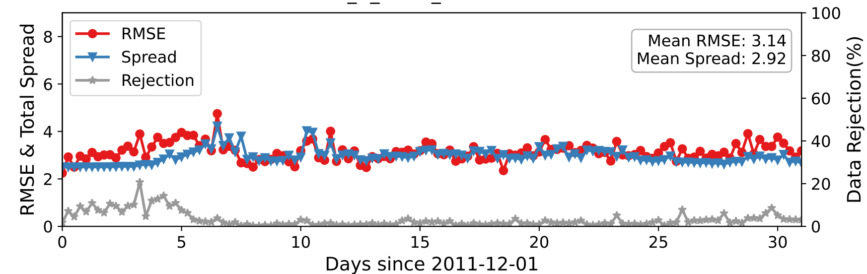
DARTEN20 — ACARS_U_WIND_COMPONENT at 450-600 hPa
