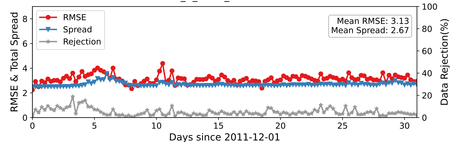
DARTEN40 — ACARS_U_WIND_COMPONENT at 450-600 hPa
