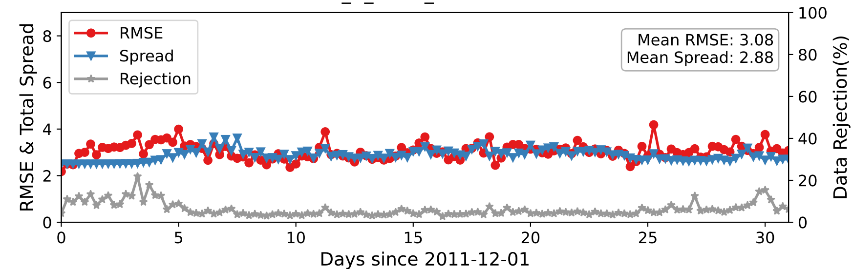
DARTEN20 — ACARS_U_WIND_COMPONENT at 600-775 hPa
