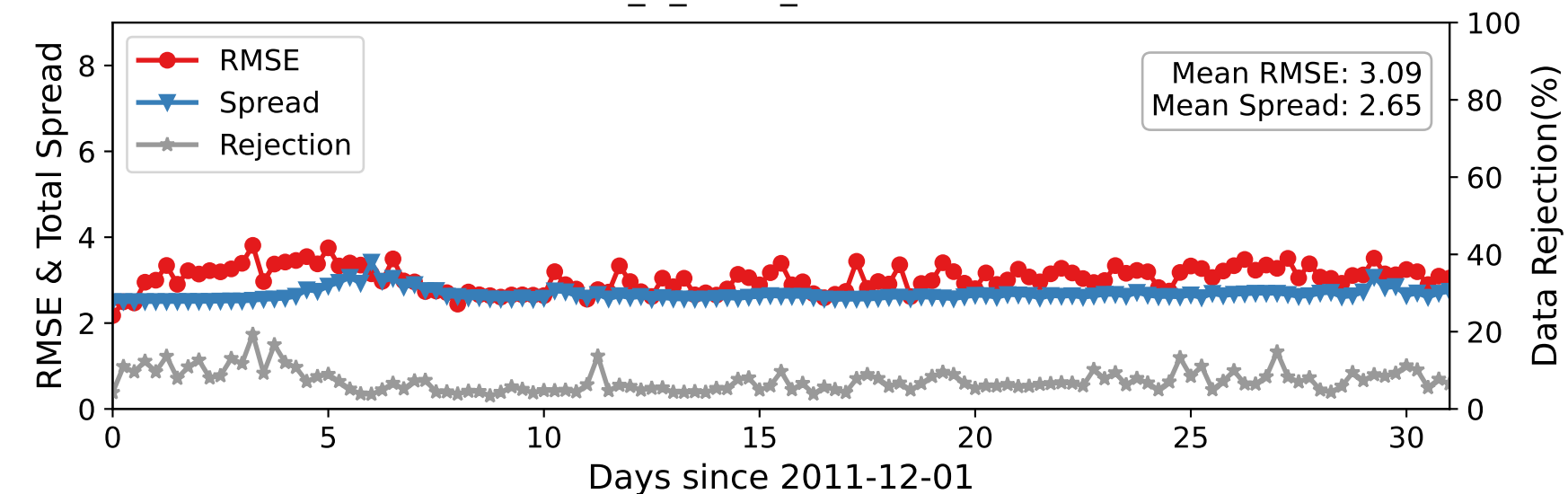
DARTEN40 — ACARS_U_WIND_COMPONENT at 600-775 hPa
