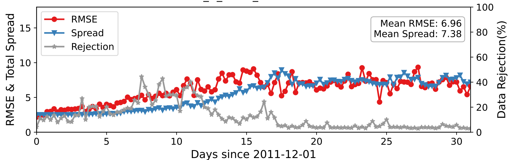
CTRLN10 — ACARS_U_WIND_COMPONENT at 600-775 hPa
