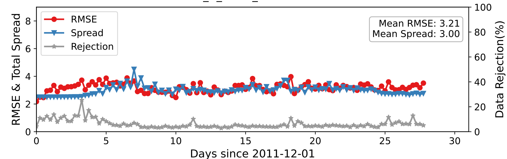
DARTEN10 — ACARS_U_WIND_COMPONENT at 600-775 hPa
