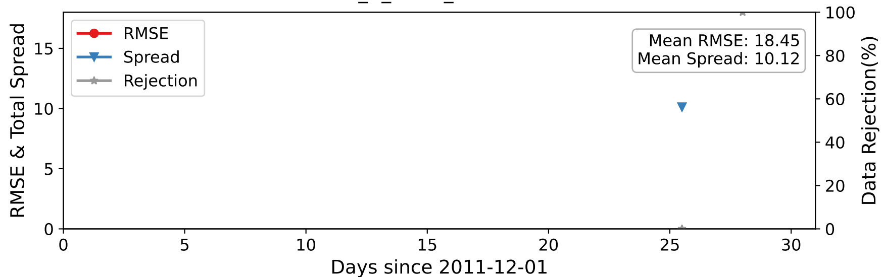
CTRLN10 — ACARS_U_WIND_COMPONENT at 75-125 hPa
