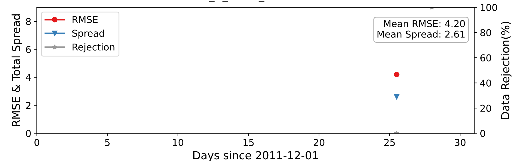
DARTEN40 — ACARS_U_WIND_COMPONENT at 75-125 hPa
