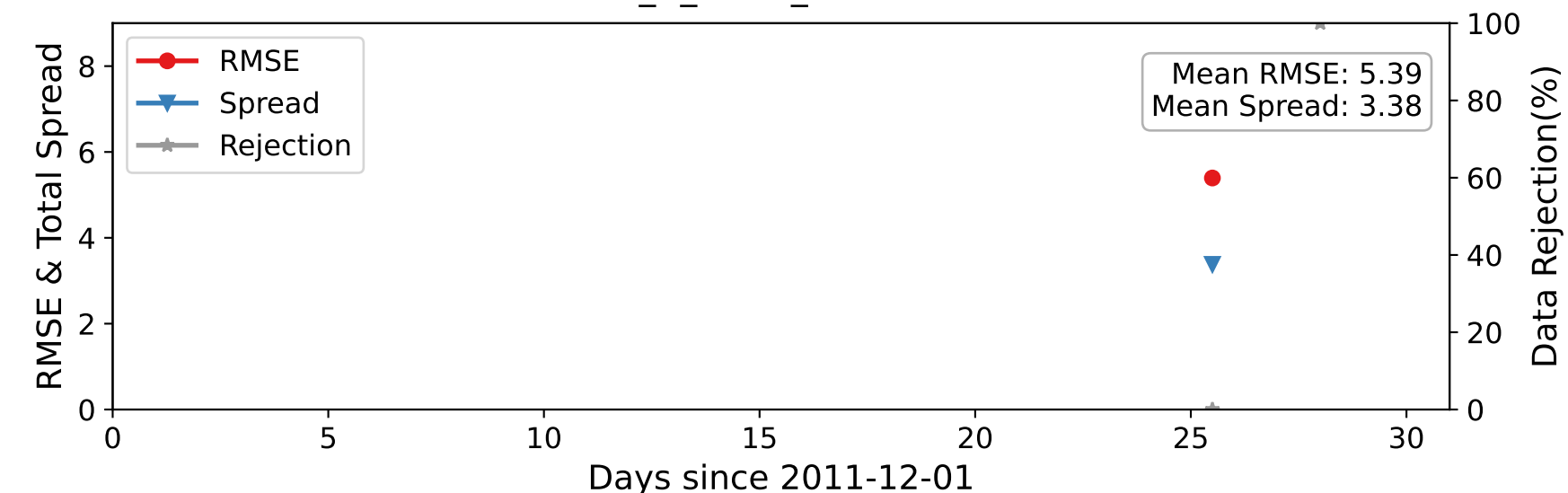
DARTEN20 — ACARS_U_WIND_COMPONENT at 75-125 hPa
