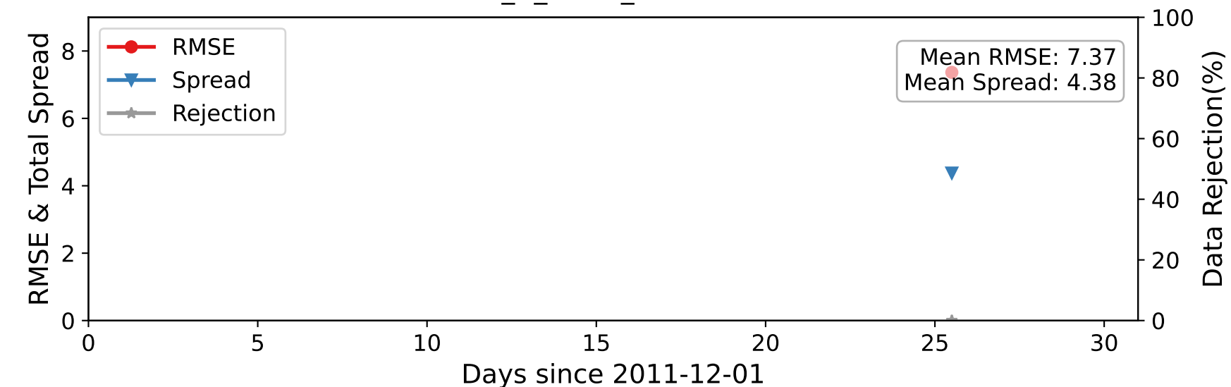
DARTEN10 — ACARS_U_WIND_COMPONENT at 75-125 hPa
