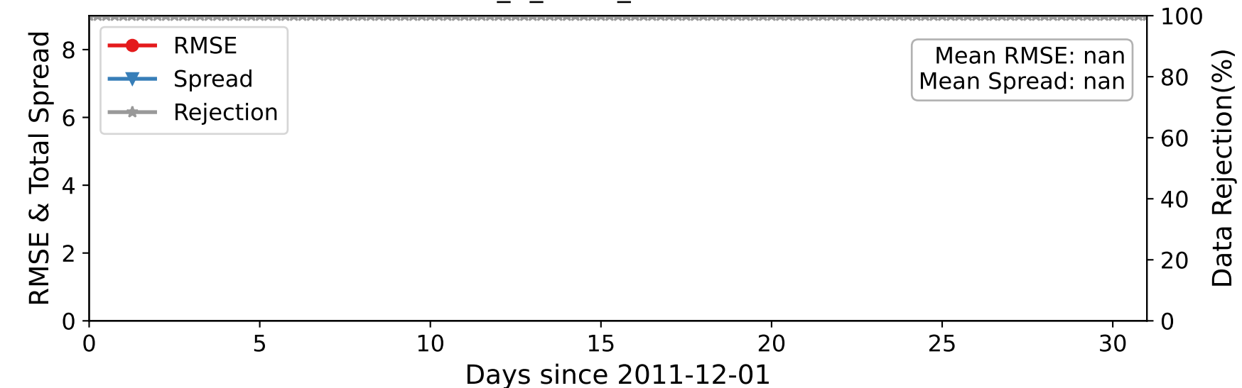
DARTEN40 — ACARS_U_WIND_COMPONENT at 775-887 hPa
