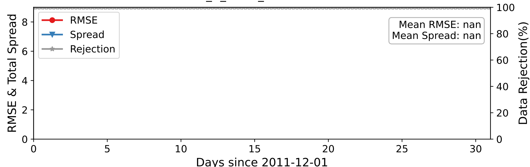
DARTEN20 — ACARS_U_WIND_COMPONENT at 962-1035 hPa
