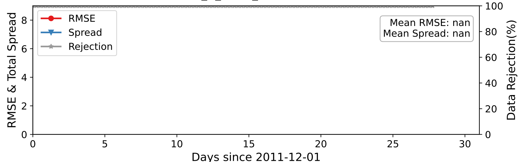
DARTEN10 — ACARS_U_WIND_COMPONENT at 962-1035 hPa
