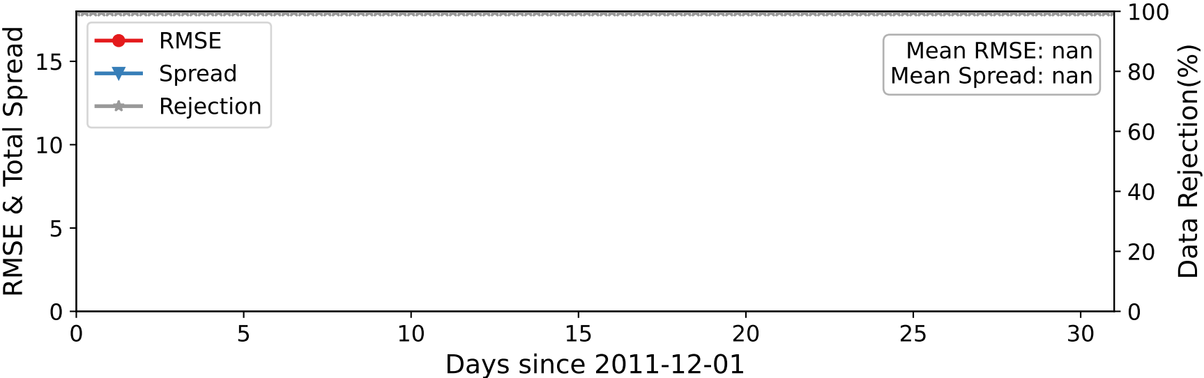
CTRLN10 — ACARS_U_WIND_COMPONENT at 962-1035 hPa
