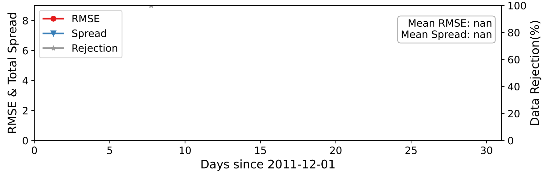
DARTEN10 — ACARS_U_WIND_COMPONENT at 15-35 hPa
