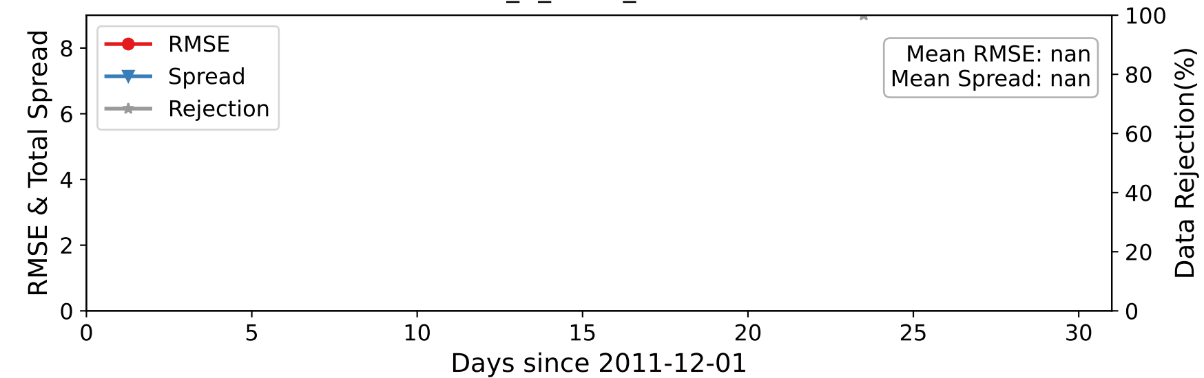
DARTEN40 — ACARS_U_WIND_COMPONENT at 2-15 hPa
