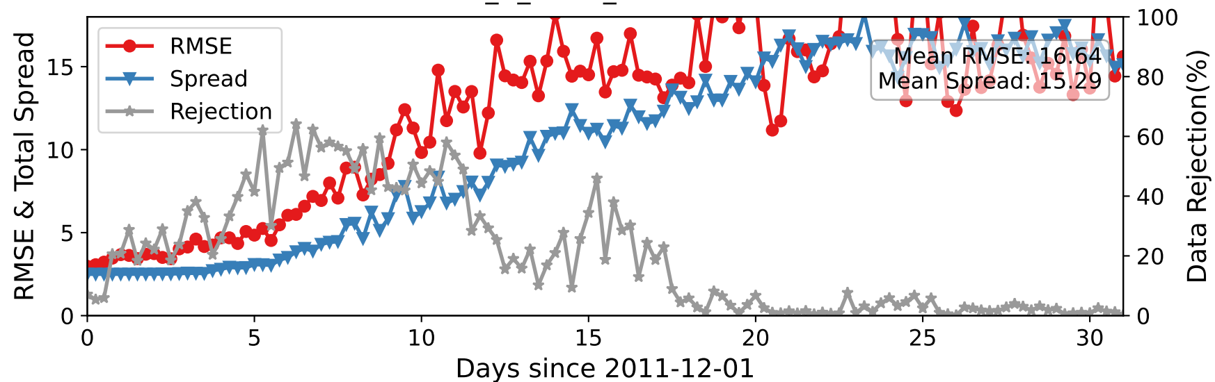
CTRLN10 — ACARS_U_WIND_COMPONENT at 275-350 hPa
