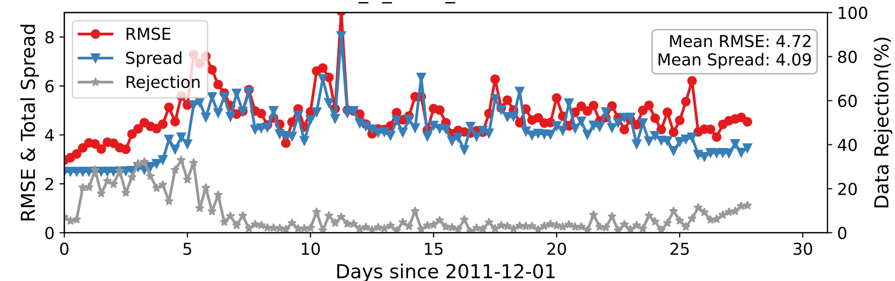
DARTEN10 — ACARS_U_WIND_COMPONENT at 275-350 hPa
