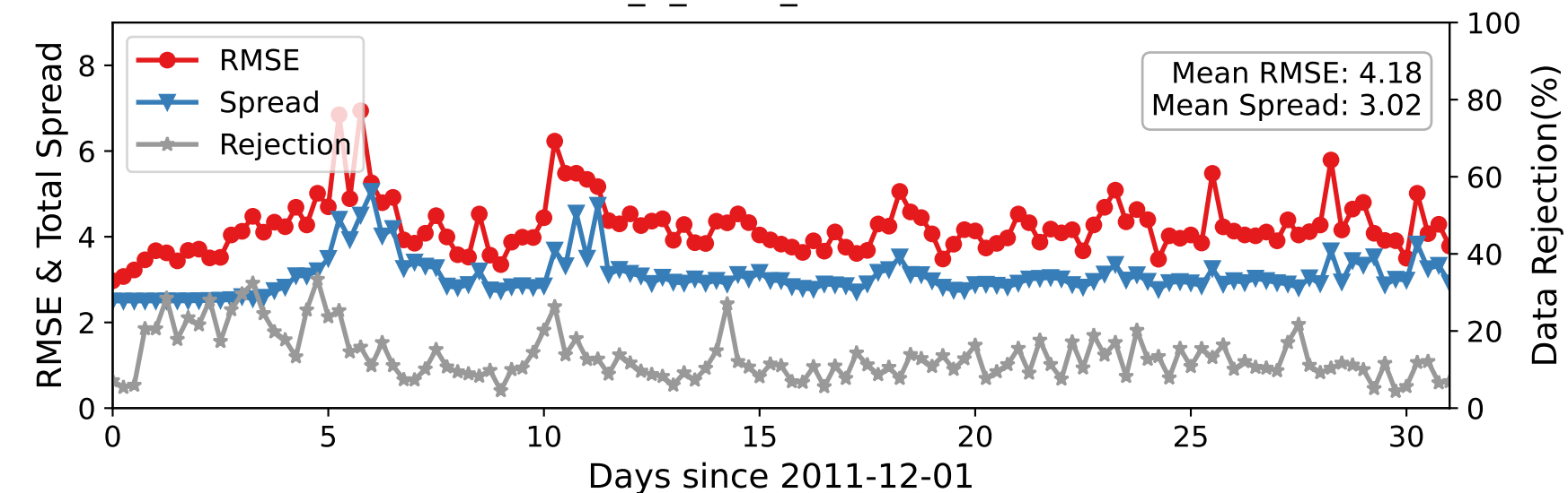
DARTEN40 — ACARS_U_WIND_COMPONENT at 275-350 hPa
