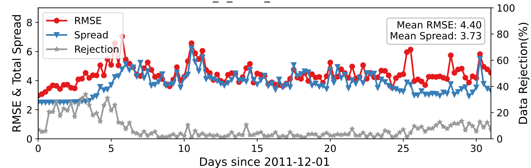
DARTEN20 — ACARS_U_WIND_COMPONENT at 275-350 hPa
