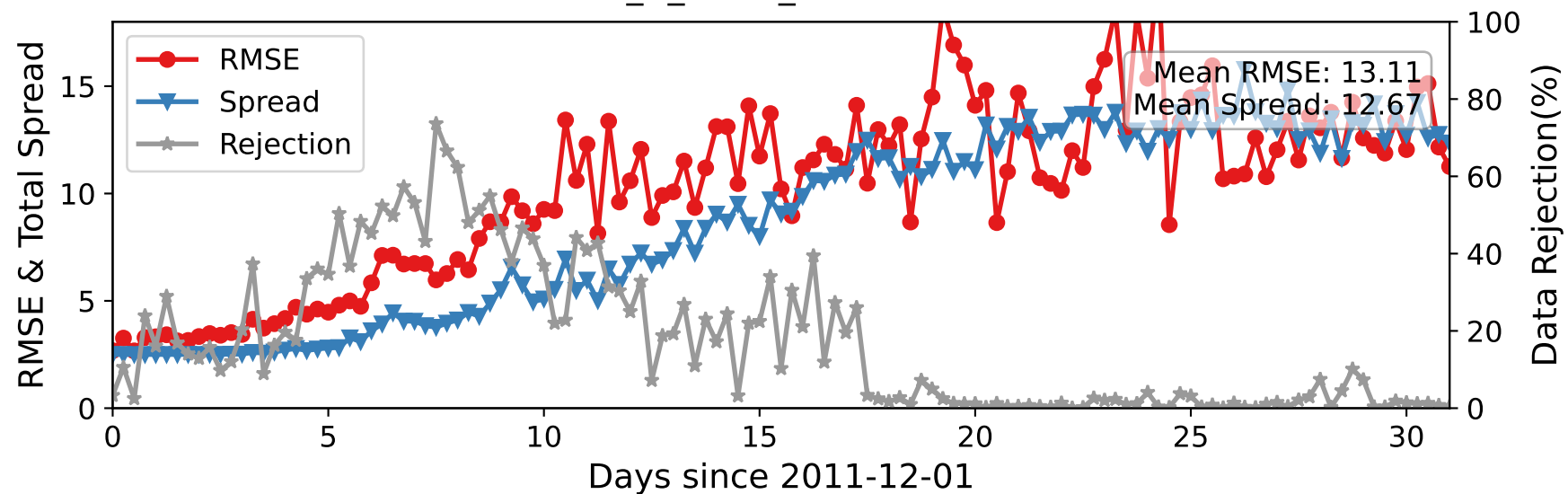
CTRLN10 — ACARS_U_WIND_COMPONENT at 350-450 hPa
