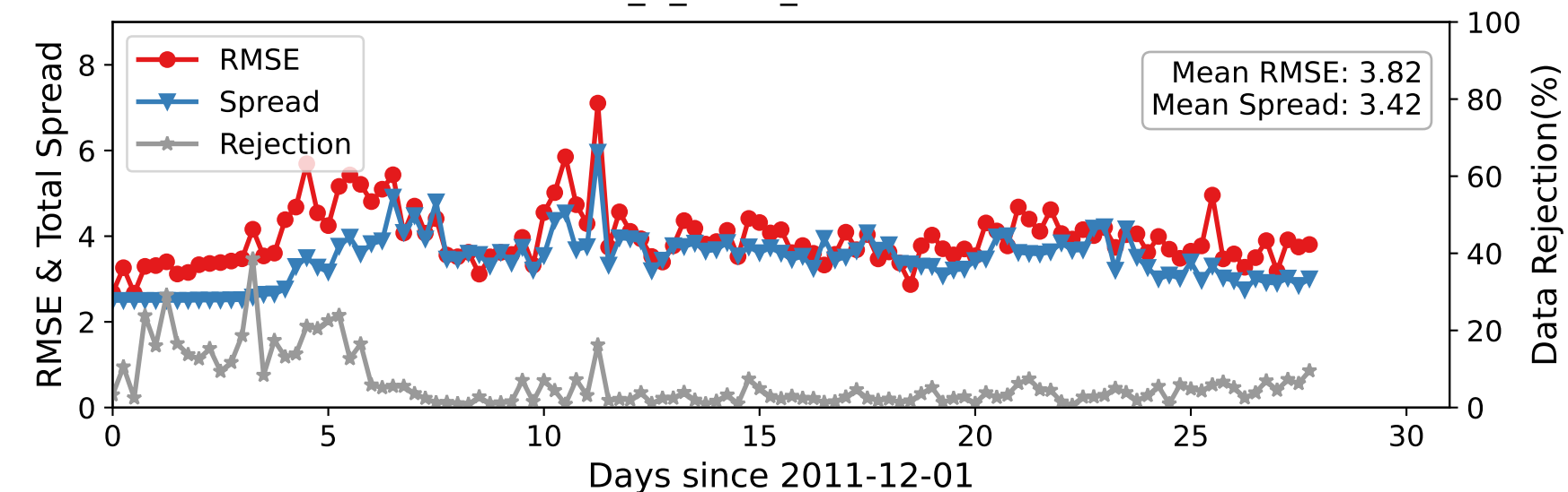
DARTEN10 — ACARS_U_WIND_COMPONENT at 350-450 hPa
