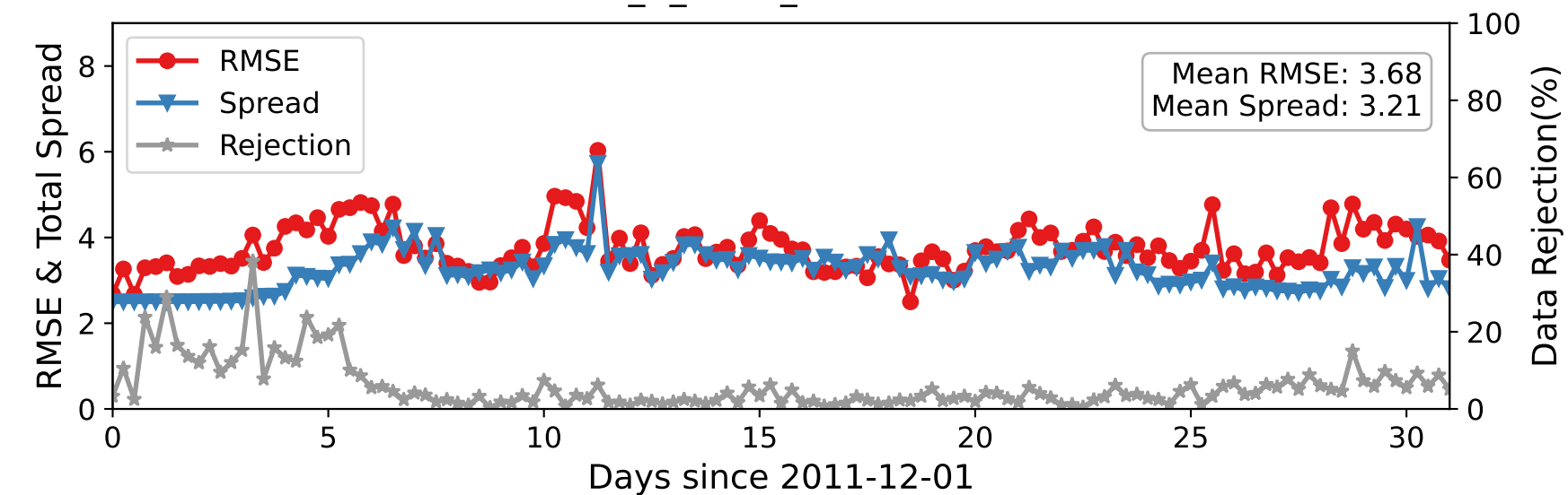
DARTEN20 — ACARS_U_WIND_COMPONENT at 350-450 hPa
