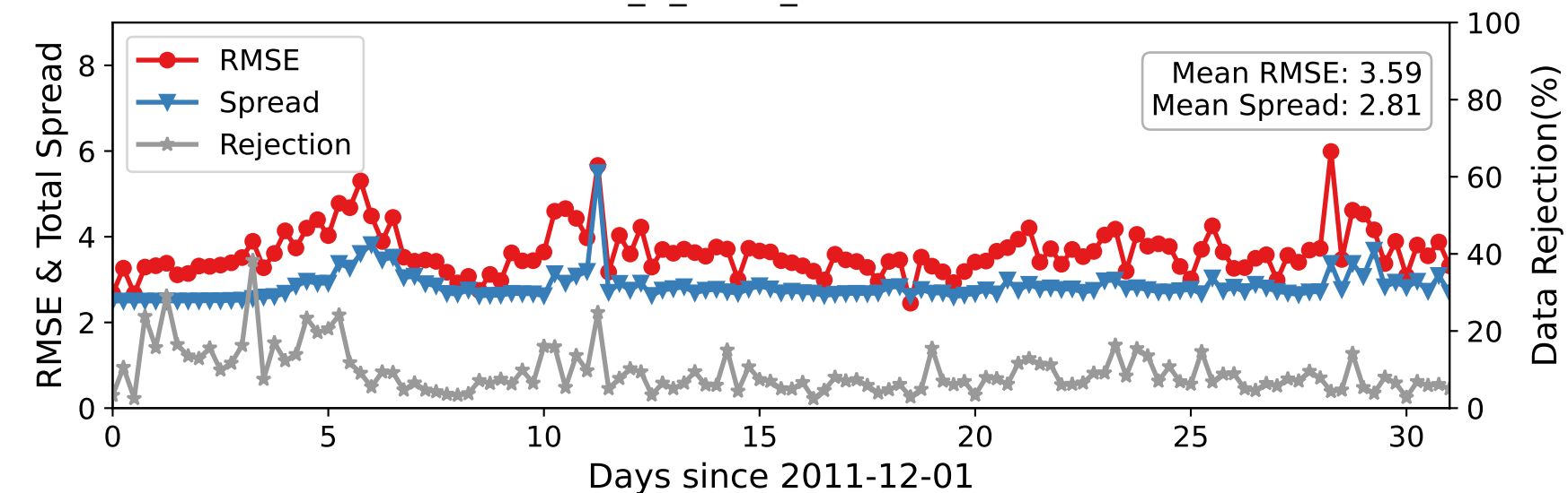
DARTEN40 — ACARS_U_WIND_COMPONENT at 350-450 hPa
