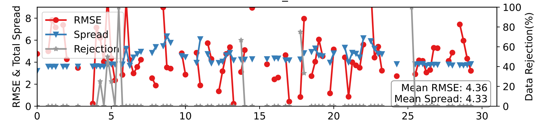
DARTEN20 — AIRCRAFT_U at 125-175 hPa
