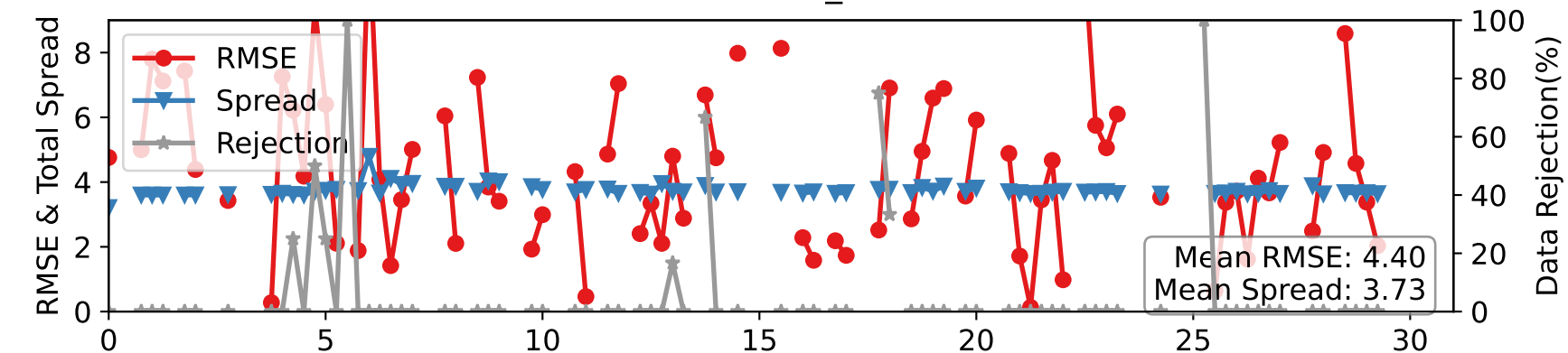
DARTEN40 — AIRCRAFT_U at 125-175 hPa
