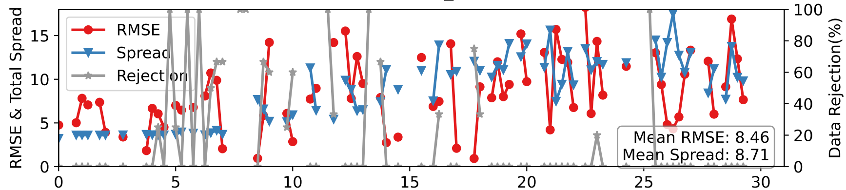
CTRLN10 — AIRCRAFT_U at 125-175 hPa
