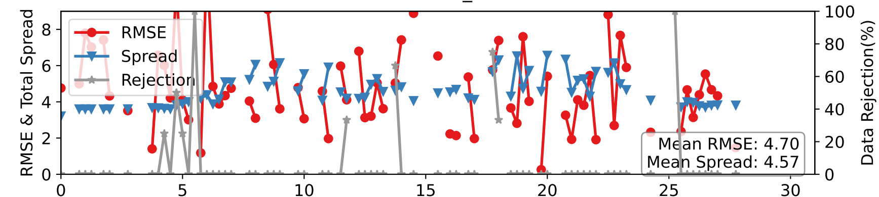
DARTEN10 — AIRCRAFT_U at 125-175 hPa
