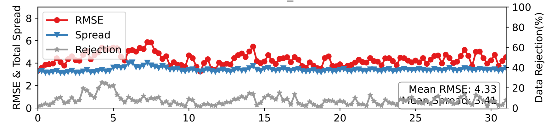
DARTEN40 — AIRCRAFT_U at 175-225 hPa
