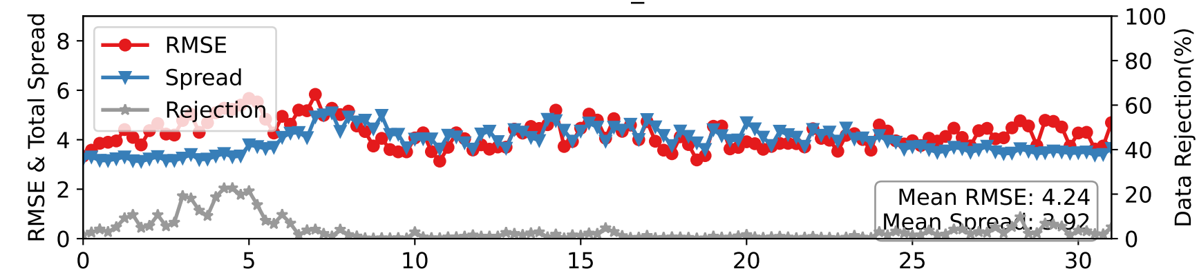
DARTEN20 — AIRCRAFT_U at 175-225 hPa
