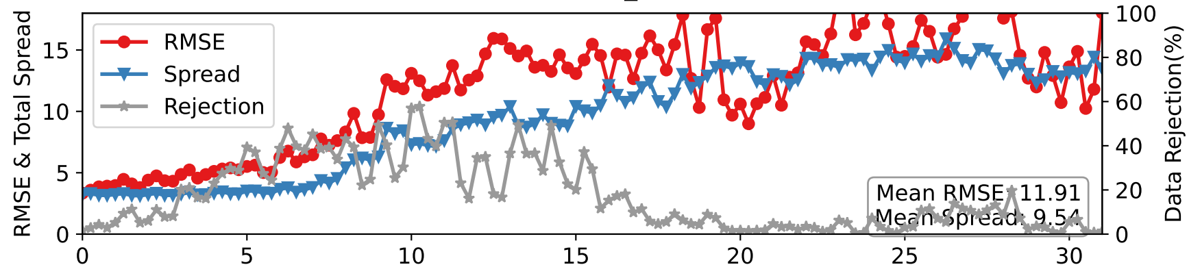
CTRLN10 — AIRCRAFT_U at 175-225 hPa
