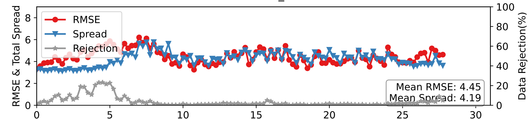
DARTEN10 — AIRCRAFT_U at 175-225 hPa
