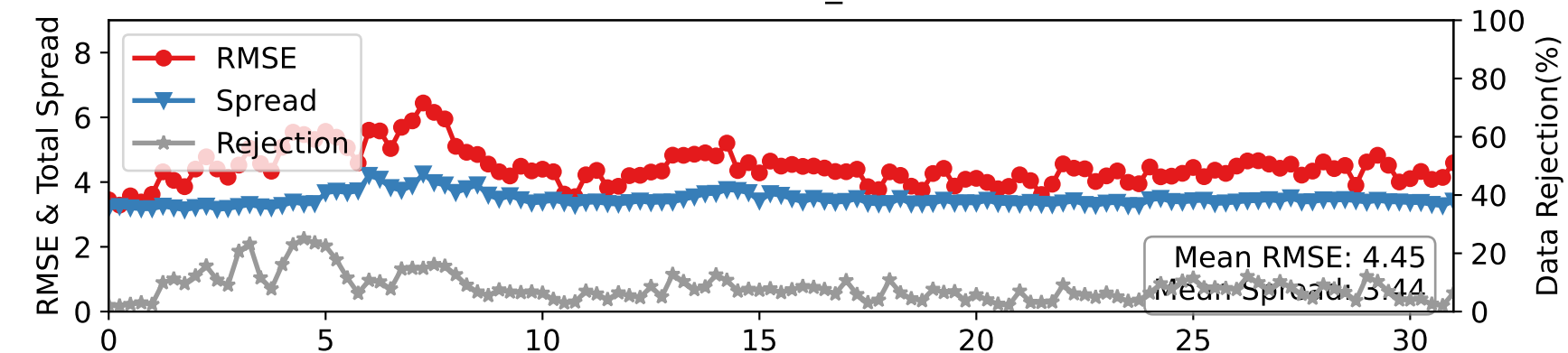
DARTEN40 — AIRCRAFT_U at 225-275 hPa
