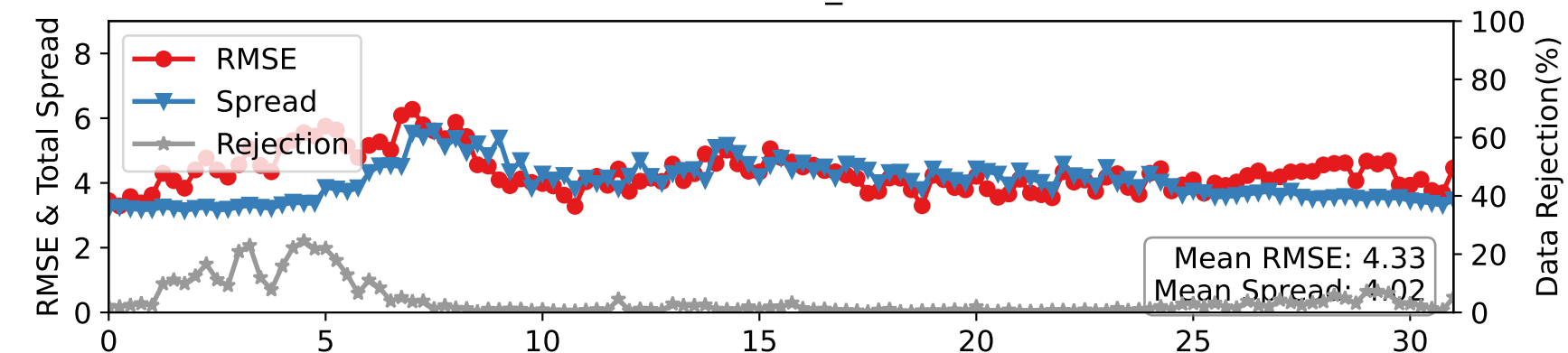
DARTEN20 — AIRCRAFT_U at 225-275 hPa
