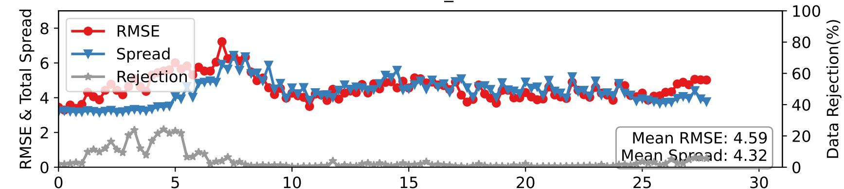
DARTEN10 — AIRCRAFT_U at 225-275 hPa
