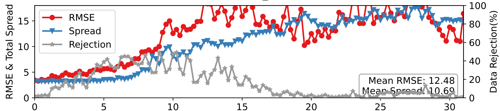
CTRLN10 — AIRCRAFT_U at 225-275 hPa
