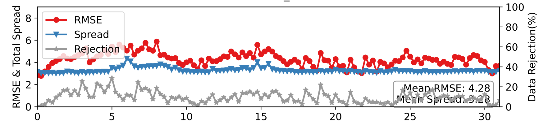
DARTEN40 — AIRCRAFT_U at 275-350 hPa
