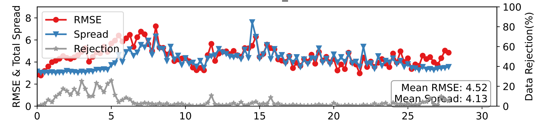
DARTEN10 — AIRCRAFT_U at 275-350 hPa
