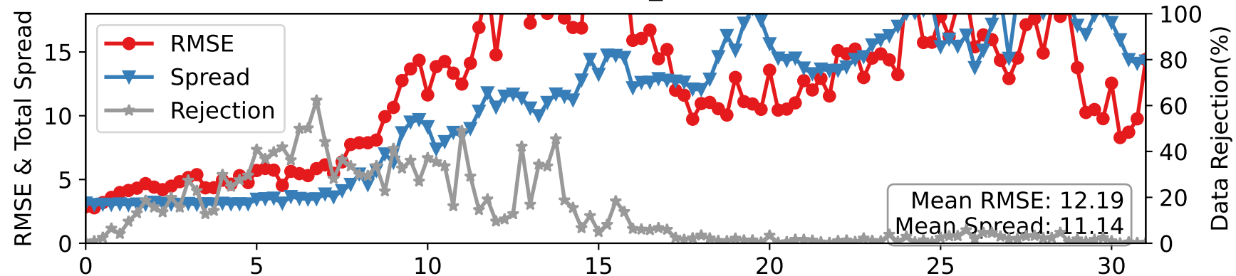
CTRLN10 — AIRCRAFT_U at 275-350 hPa
