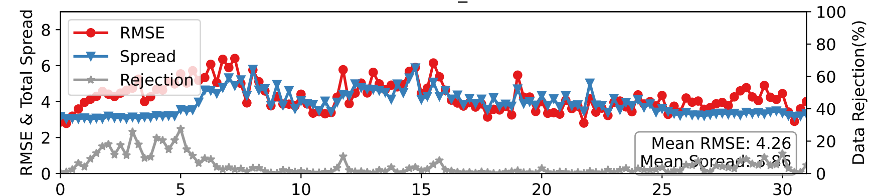
DARTEN20 — AIRCRAFT_U at 275-350 hPa
