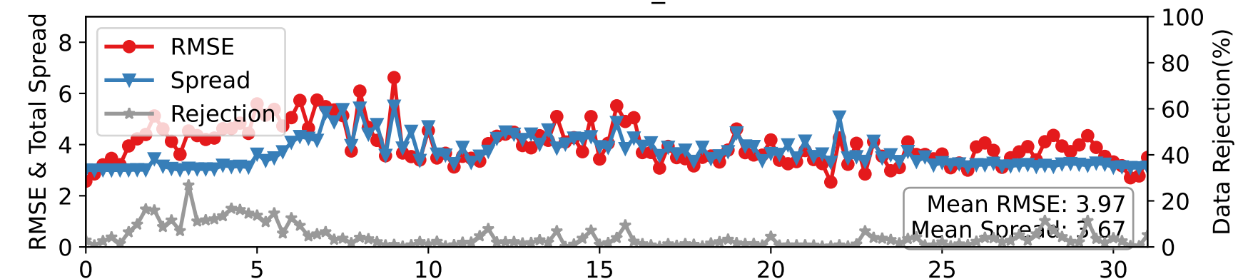
DARTEN20 — AIRCRAFT_U at 350-450 hPa
