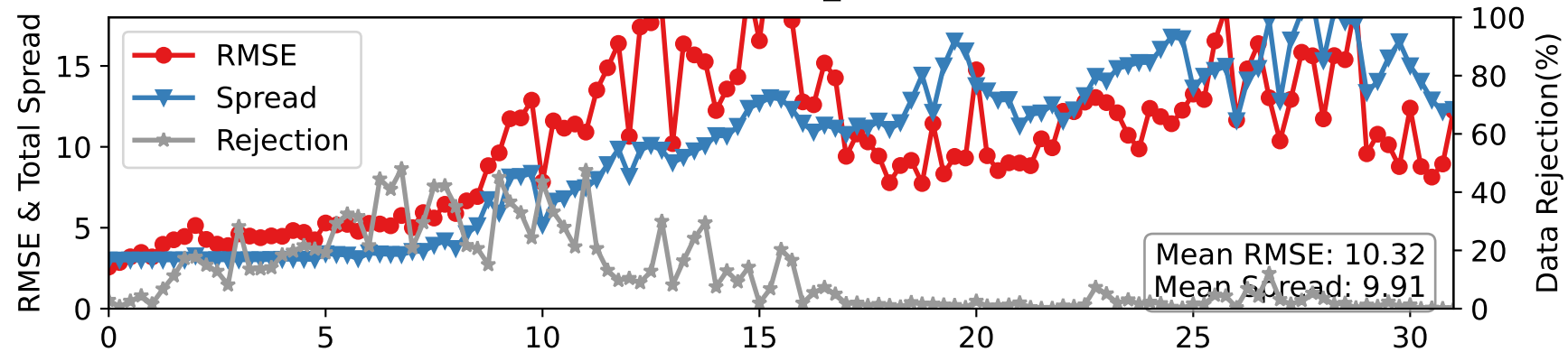
CTRLN10 — AIRCRAFT_U at 350-450 hPa
