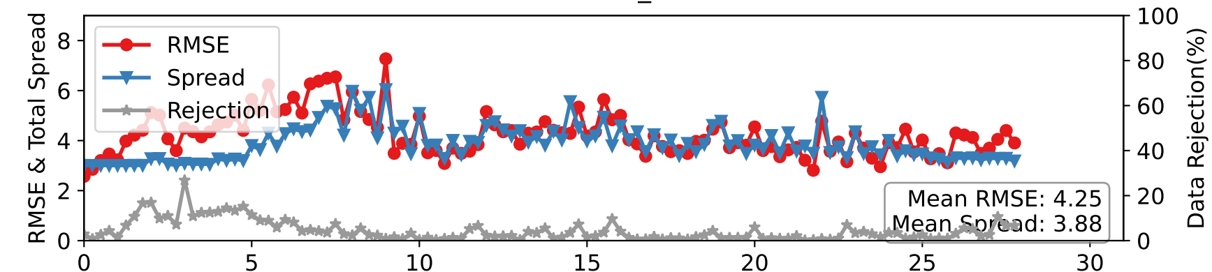
DARTEN10 — AIRCRAFT_U at 350-450 hPa
