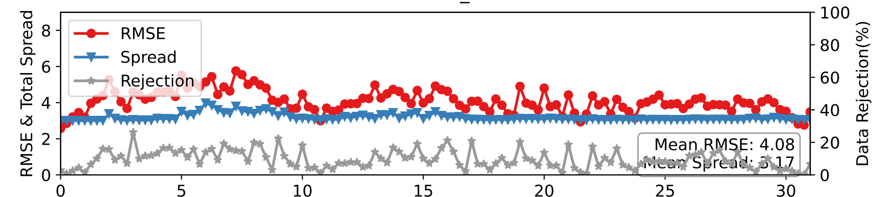
DARTEN40 — AIRCRAFT_U at 350-450 hPa
