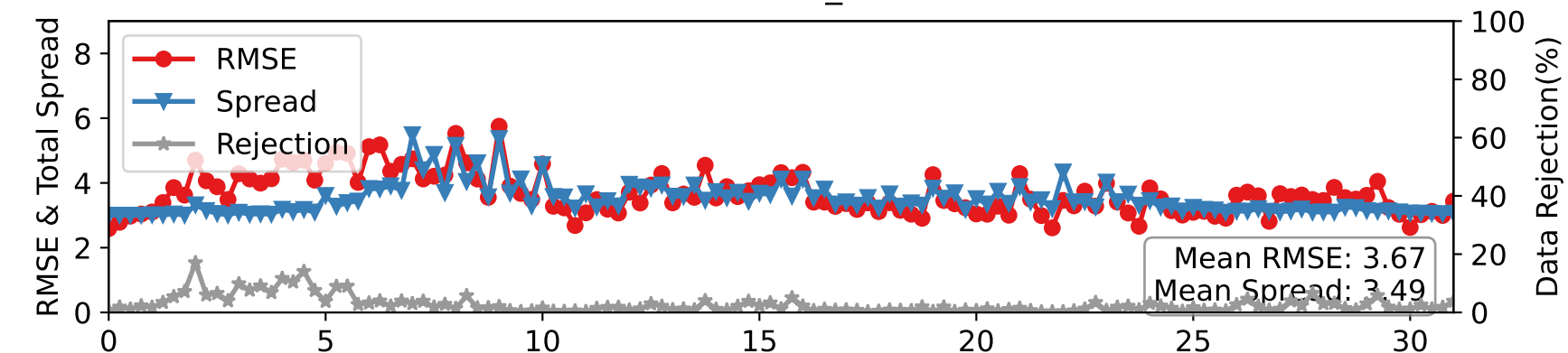
DARTEN20 — AIRCRAFT_U at 450-600 hPa
