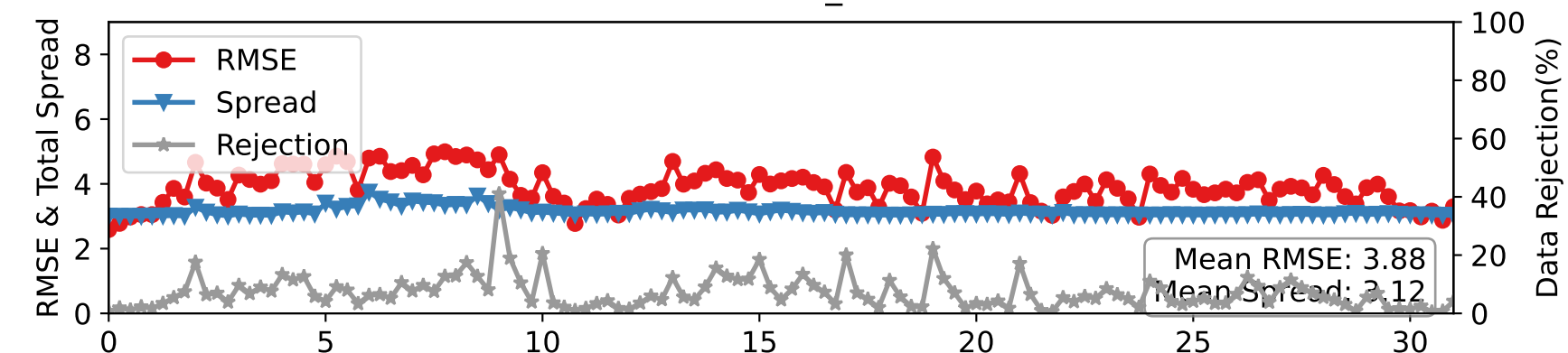
DARTEN40 — AIRCRAFT_U at 450-600 hPa
