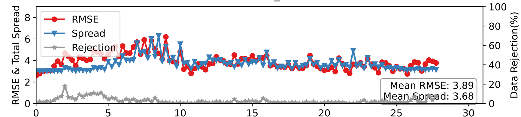
DARTEN10 — AIRCRAFT_U at 450-600 hPa
