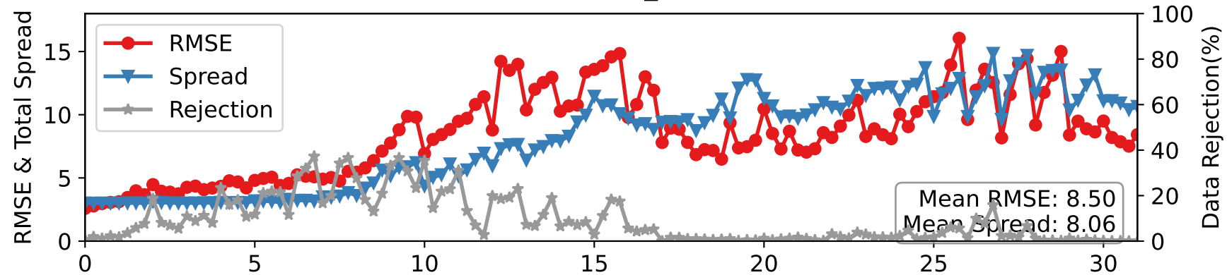
CTRLN10 — AIRCRAFT_U at 450-600 hPa
