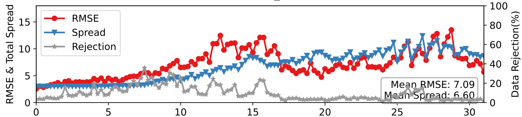
CTRLN10 — AIRCRAFT_U at 600-775 hPa
