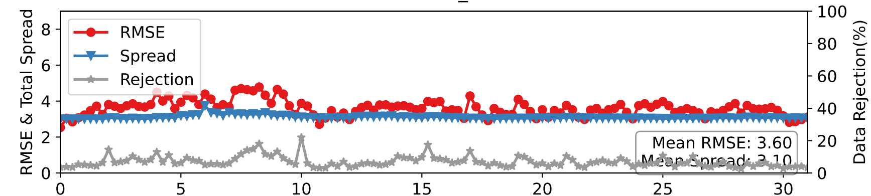
DARTEN40 — AIRCRAFT_U at 600-775 hPa
