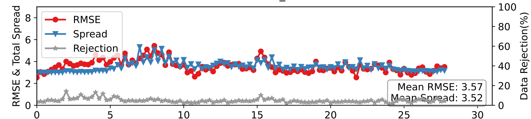
DARTEN10 — AIRCRAFT_U at 600-775 hPa
