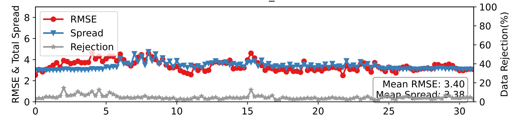
DARTEN20 — AIRCRAFT_U at 600-775 hPa
