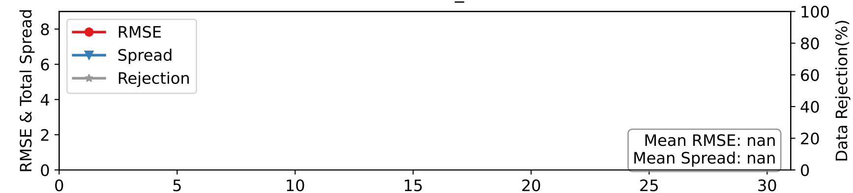
DARTEN20 — AIRCRAFT_U at 75-125 hPa
