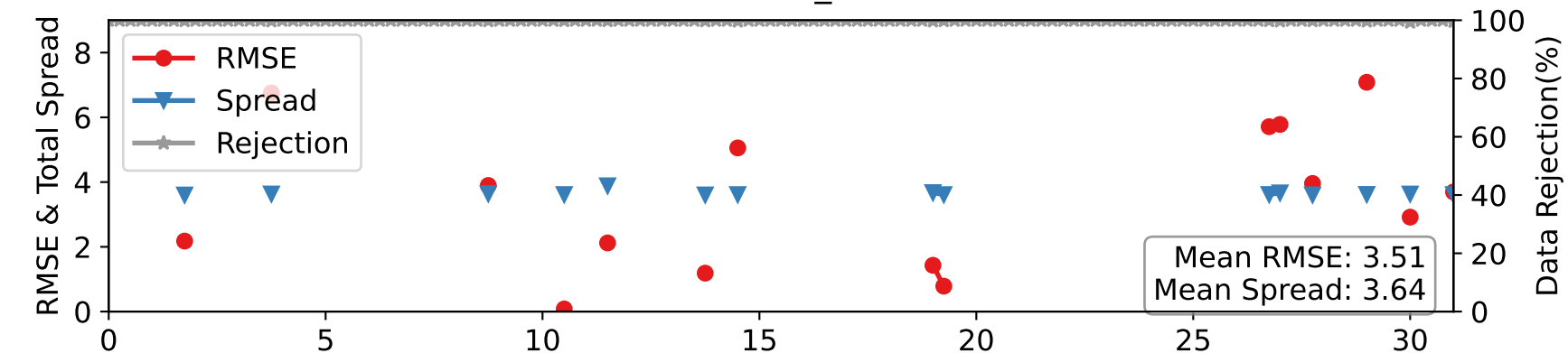
DARTEN40 — AIRCRAFT_U at 962-1035 hPa
