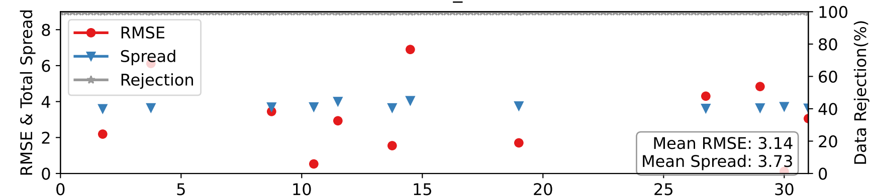
DARTEN20 — AIRCRAFT_U at 962-1035 hPa
