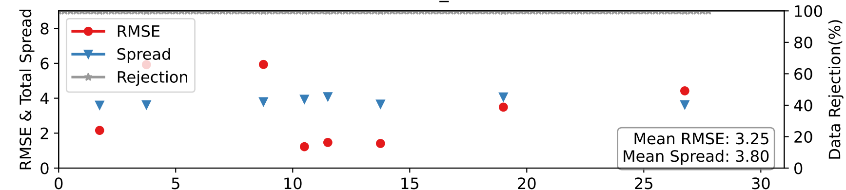
DARTEN10 — AIRCRAFT_U at 962-1035 hPa
