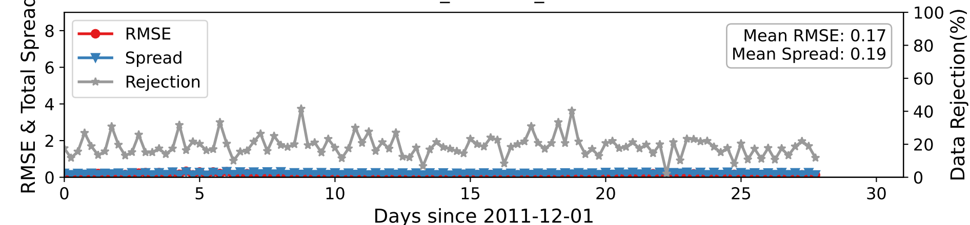
DARTEN20 — RADIOSONDE_SPECIFIC_HUMIDITY at 350-450 hPa
