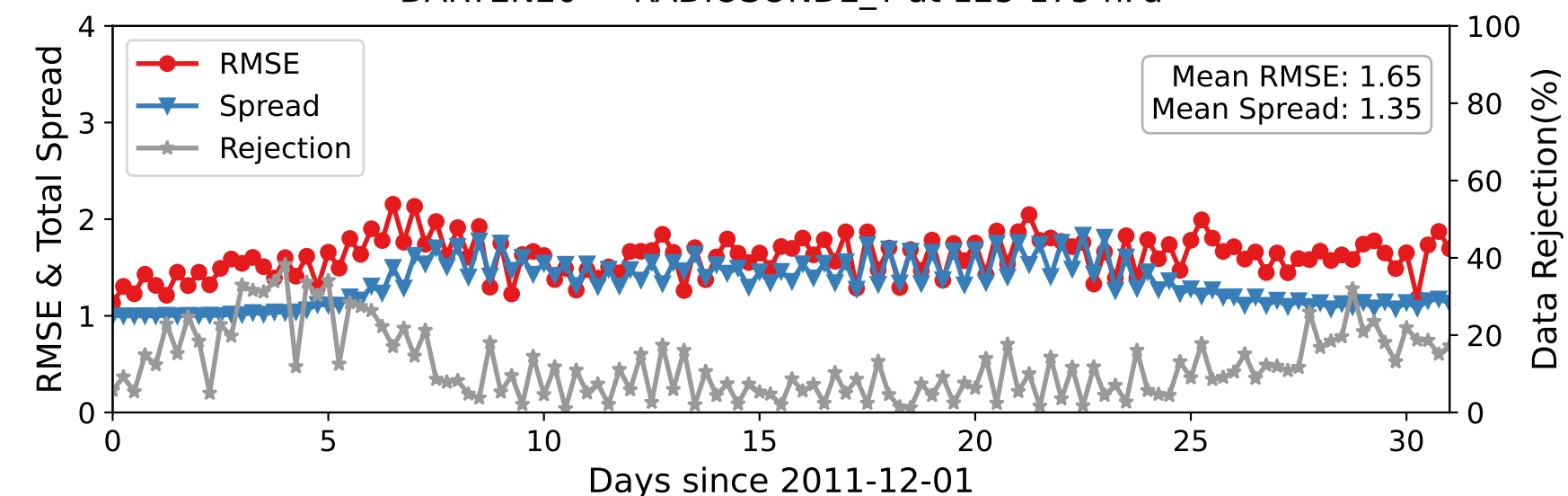
DARTEN20 — RADIOSONDE_T at 125-175 hPa
