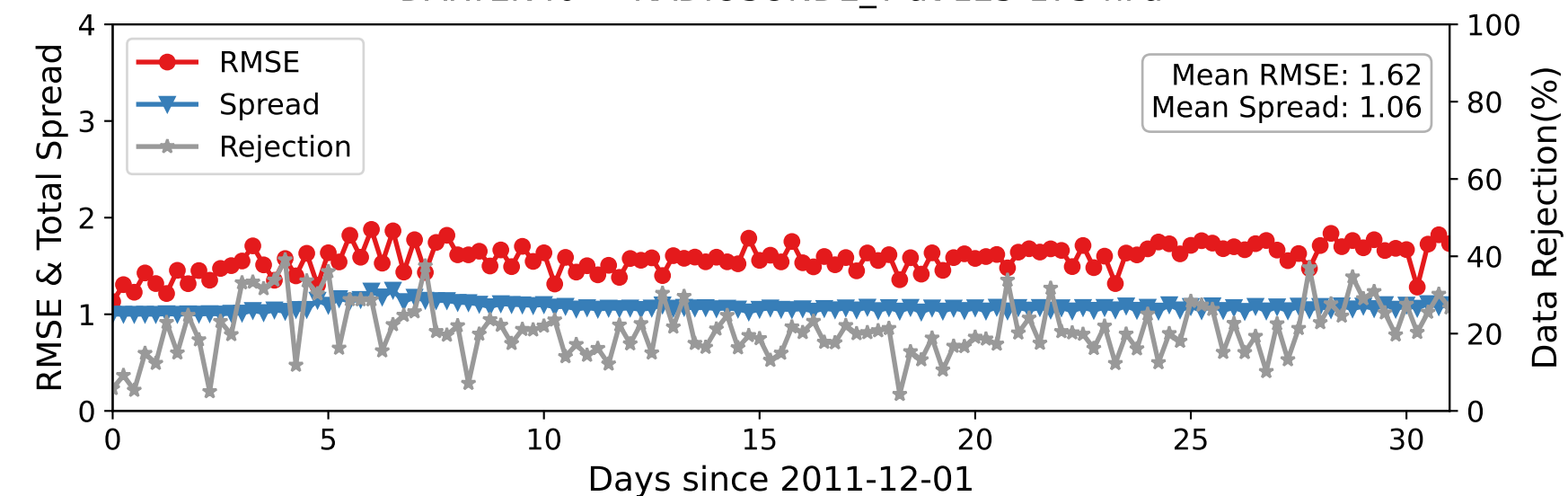
DARTEN40 — RADIOSONDE_T at 125-175 hPa
