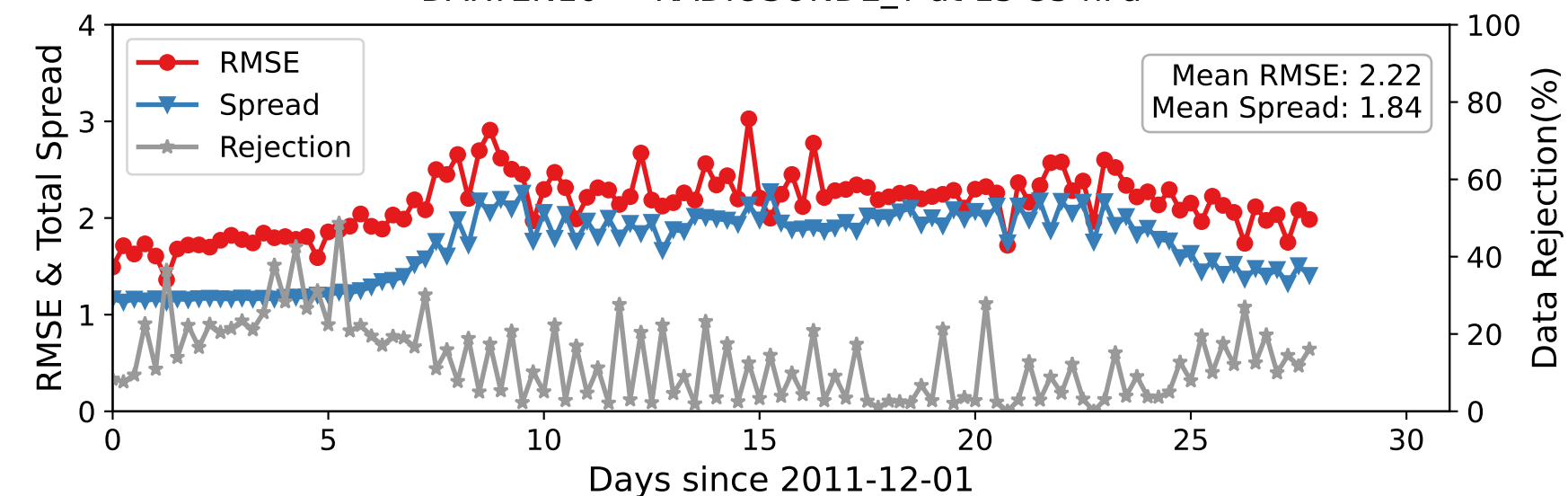
DARTEN10 — RADIOSONDE_T at 15-35 hPa
