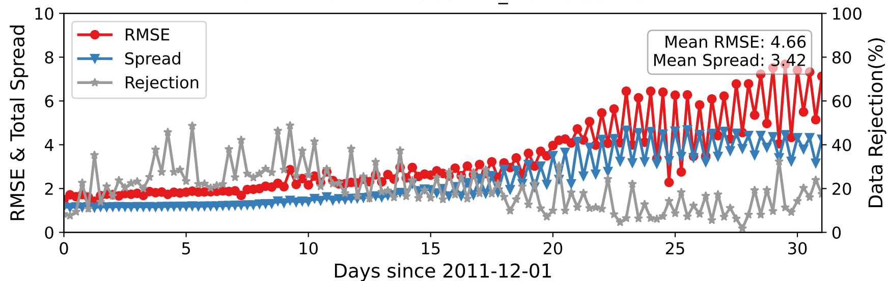
CTRLN10 — RADIOSONDE_T at 15-35 hPa
