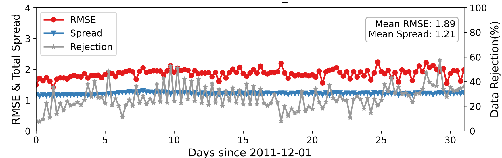
DARTEN40 — RADIOSONDE_T at 15-35 hPa
