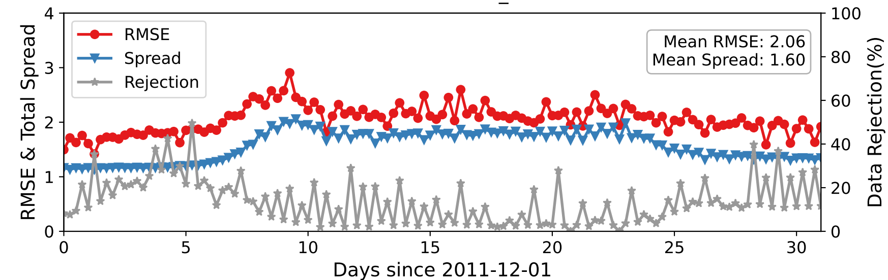
DARTEN20 — RADIOSONDE_T at 15-35 hPa
