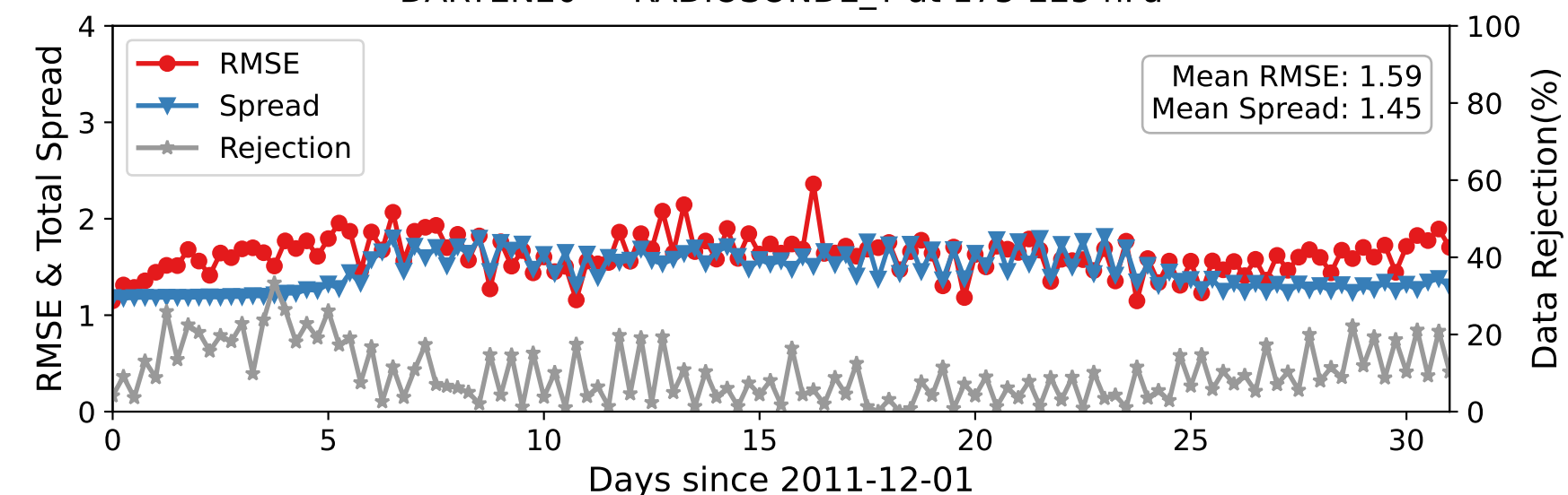
DARTEN20 — RADIOSONDE_T at 175-225 hPa
