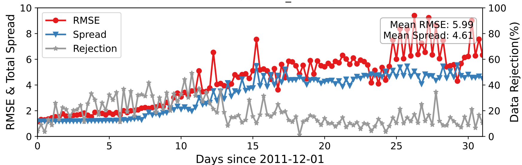
CTRLN10 — RADIOSONDE_T at 175-225 hPa
