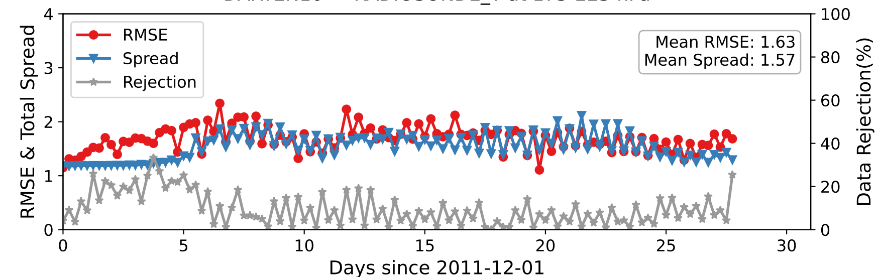
DARTEN10 — RADIOSONDE_T at 175-225 hPa
