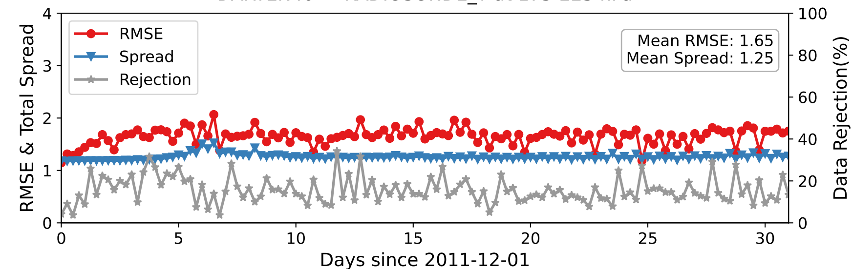
DARTEN40 — RADIOSONDE_T at 175-225 hPa
