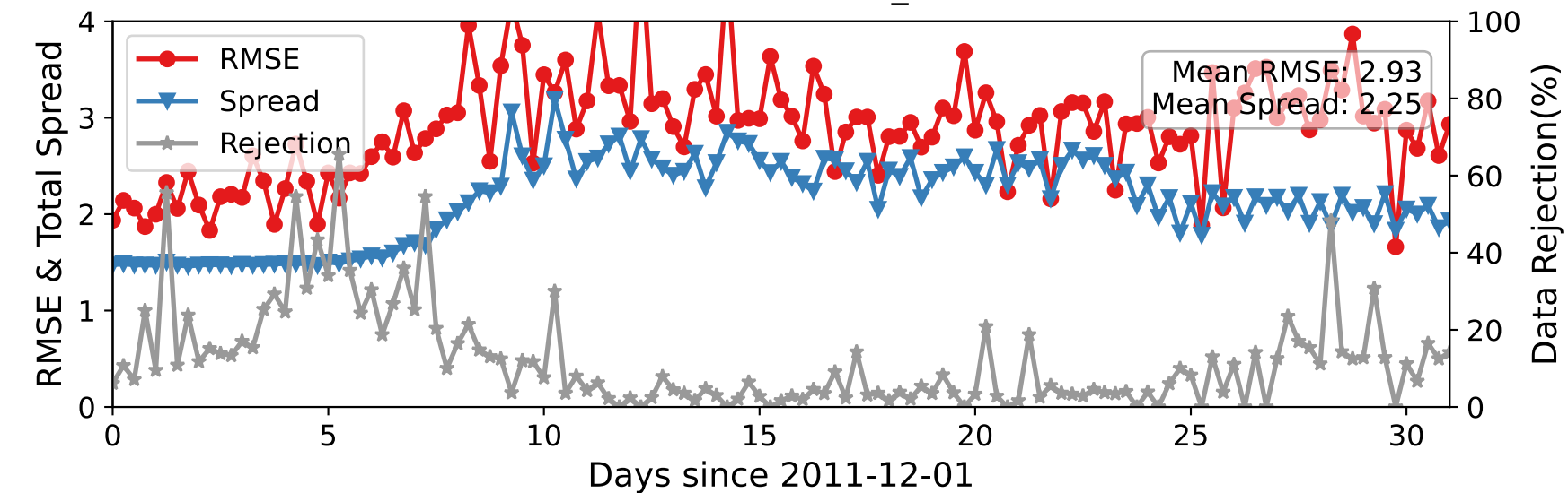
DARTEN20 — RADIOSONDE_T at 2-15 hPa
