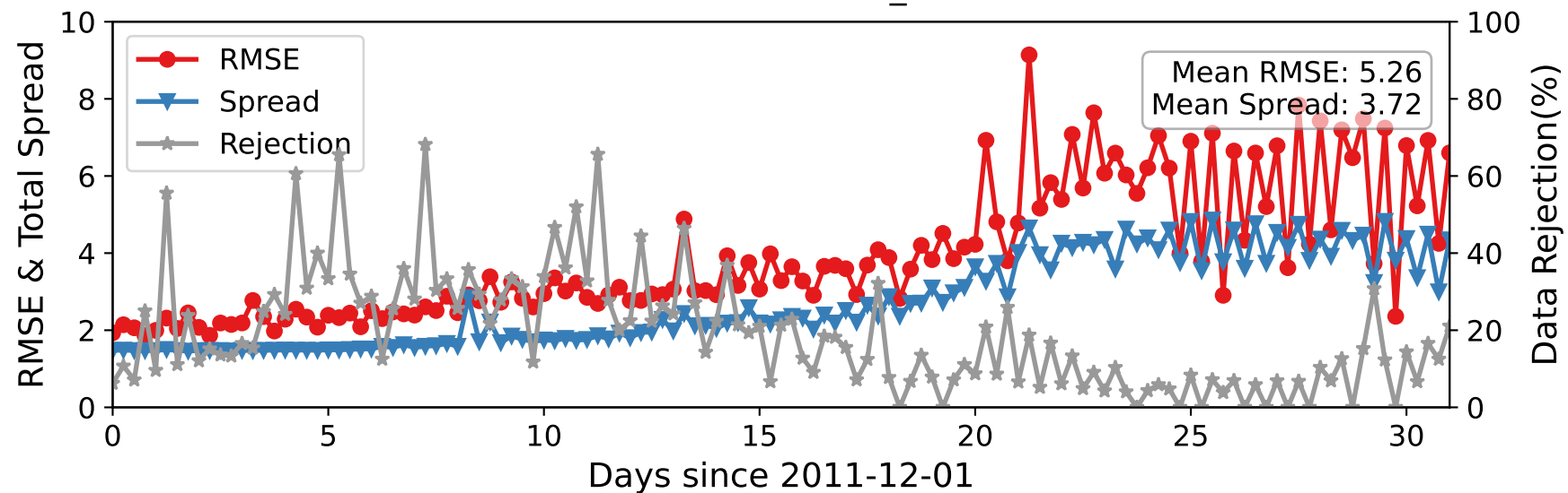
CTRLLEN10 — RADIOSONDE_T at 2-15 hPa
