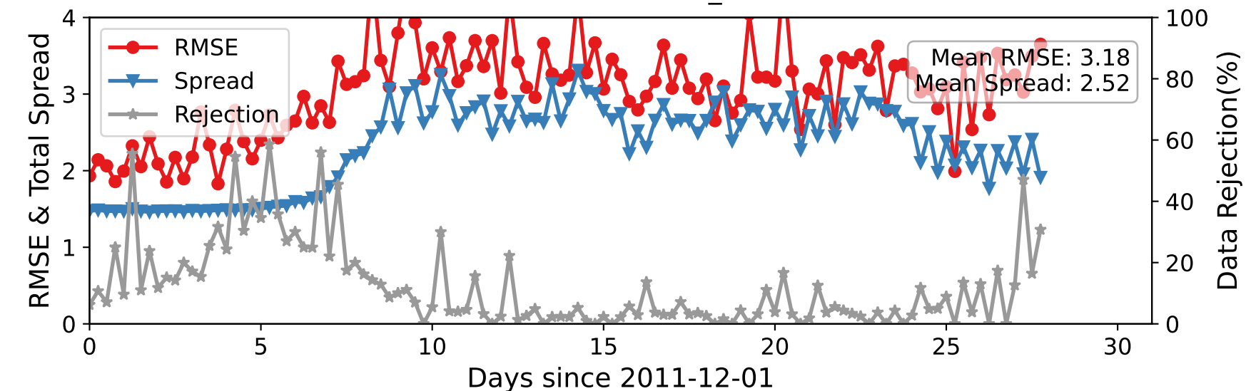
DARTEN10 — RADIOSONDE_T at 2-15 hPa
