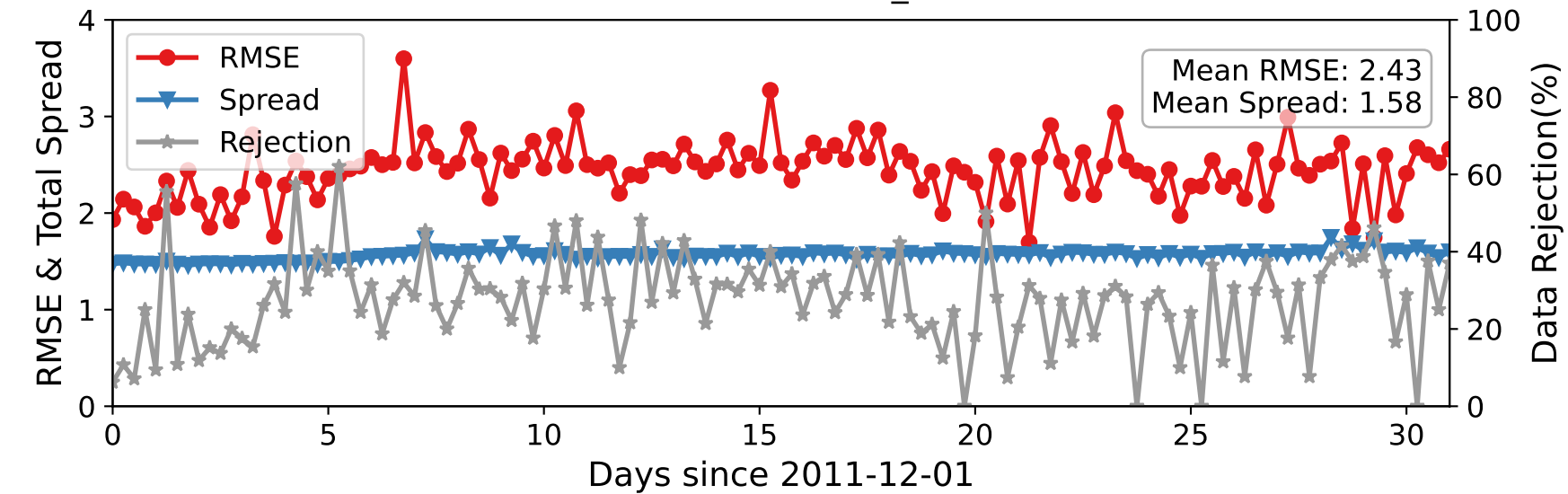
DARTEN40 — RADIOSONDE_T at 2-15 hPa
