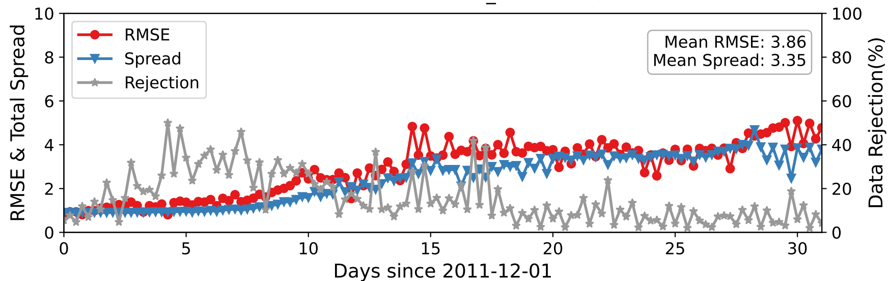
CTRLN10 — RADIOSONDE_T at 275-350 hPa
