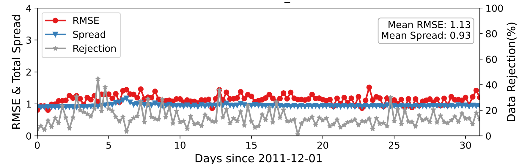
DARTEN40 — RADIOSONDE_T at 275-350 hPa
