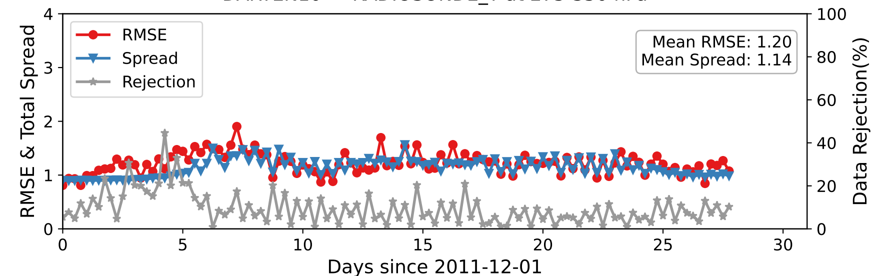
DARTEN10 — RADIOSONDE_T at 275-350 hPa
