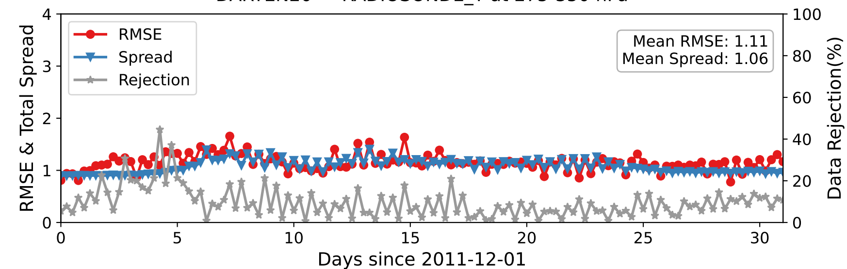
DARTEN20 — RADIOSONDE_T at 275-350 hPa
