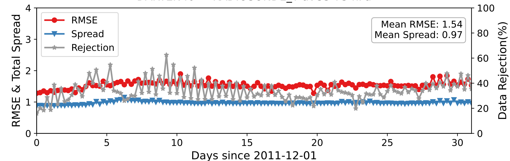
DARTEN40 — RADIOSONDE_T at 35-75 hPa
