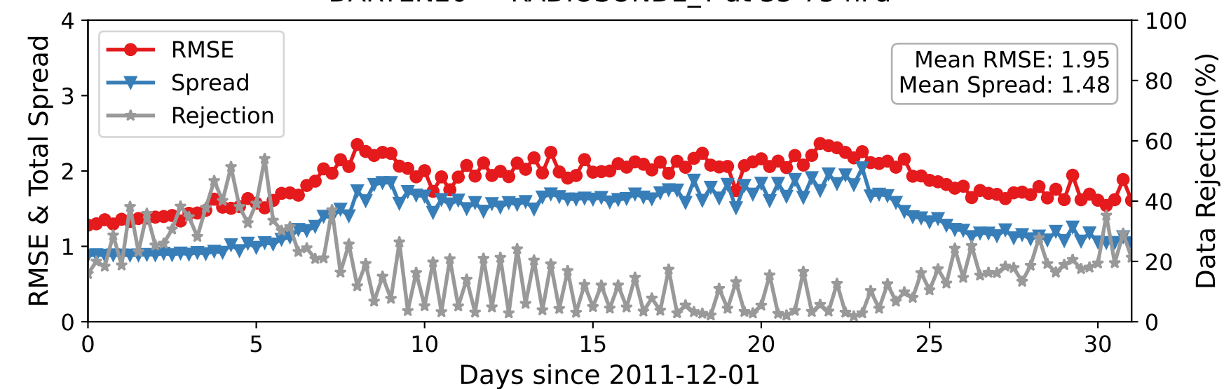
DARTEN20 — RADIOSONDE_T at 35-75 hPa
