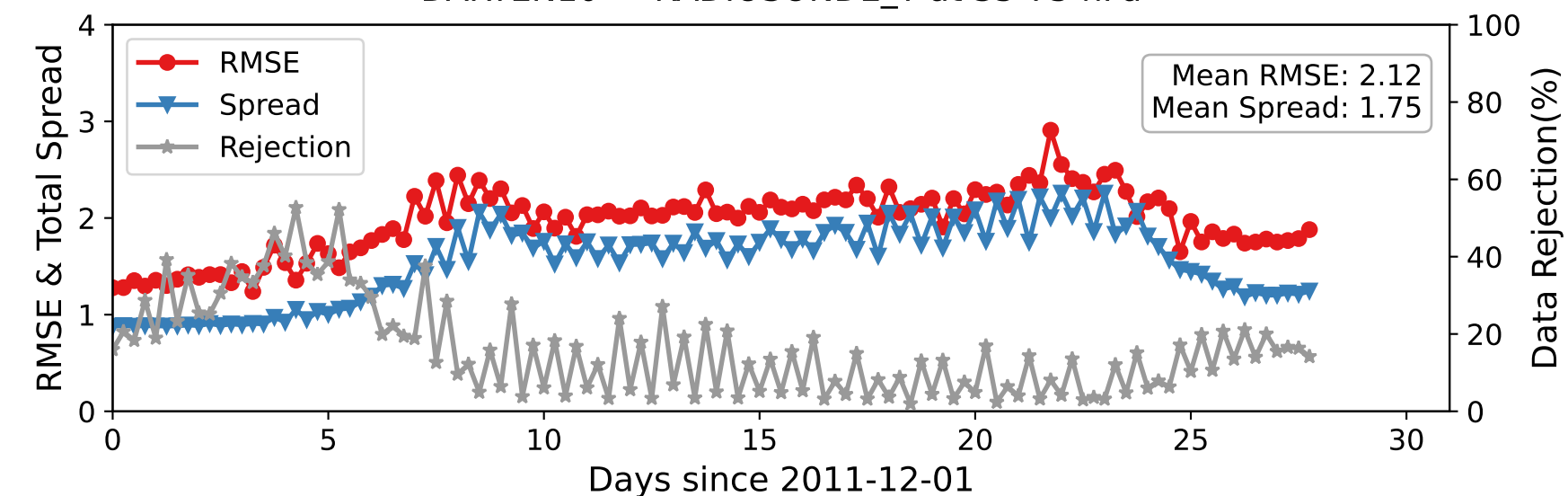
DARTEN10 — RADIOSONDE_T at 35-75 hPa
