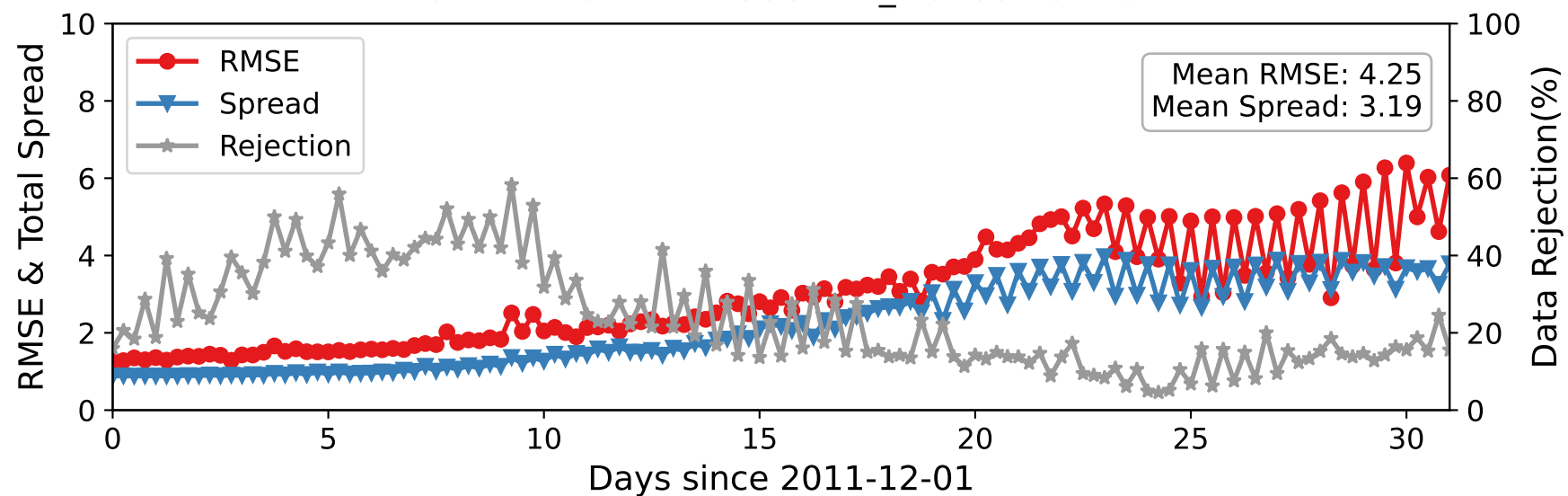
CTRLLEN10 — RADIOSONDE_T at 35-75 hPa
