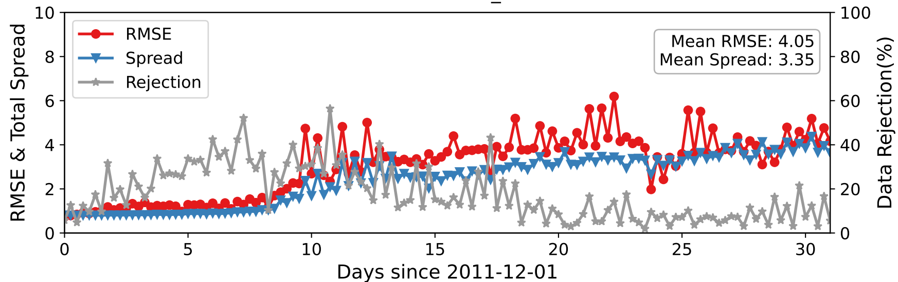
CTRLN10 — RADIOSONDE_T at 350-450 hPa
