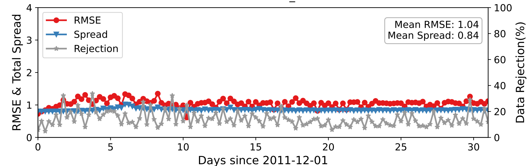
DARTEN40 — RADIOSONDE_T at 350-450 hPa
