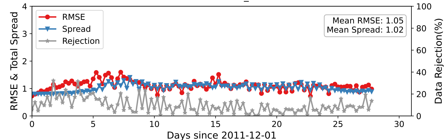
DARTEN10 — RADIOSONDE_T at 350-450 hPa
