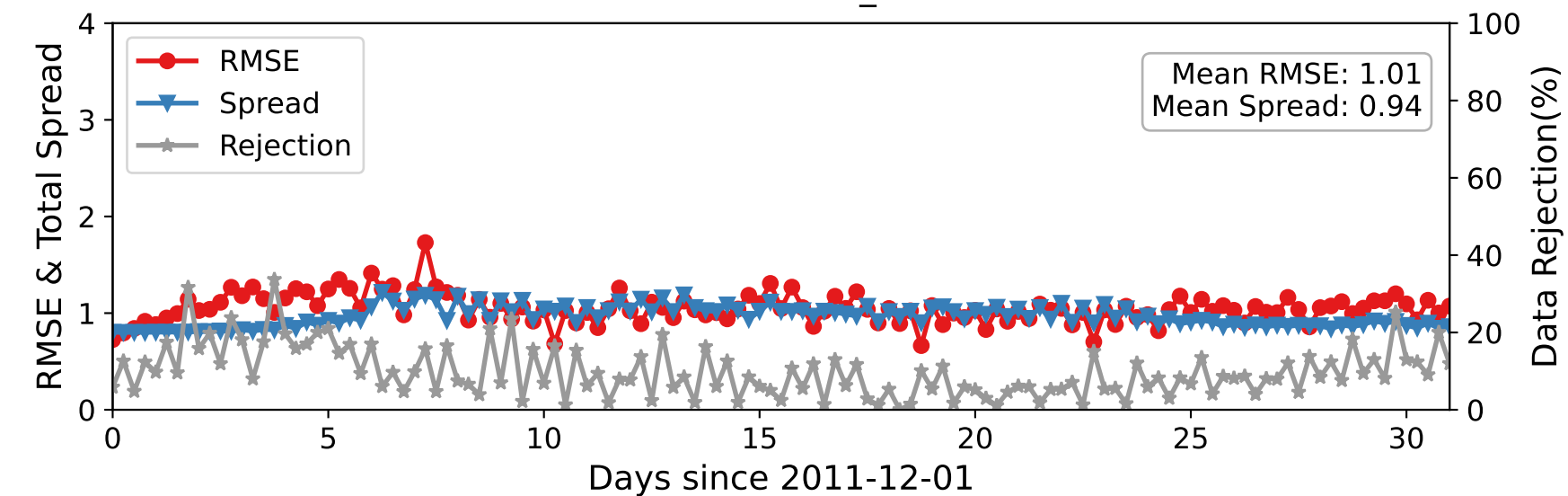
DARTEN20 — RADIOSONDE_T at 350-450 hPa
