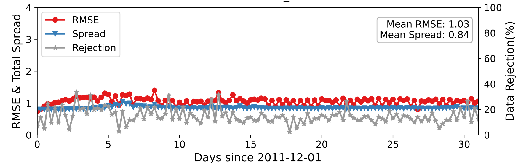
DARTEN40 — RADIOSONDE_T at 450-600 hPa
