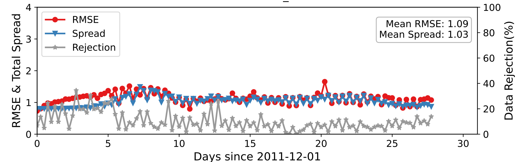
DARTEN10 — RADIOSONDE_T at 450-600 hPa
