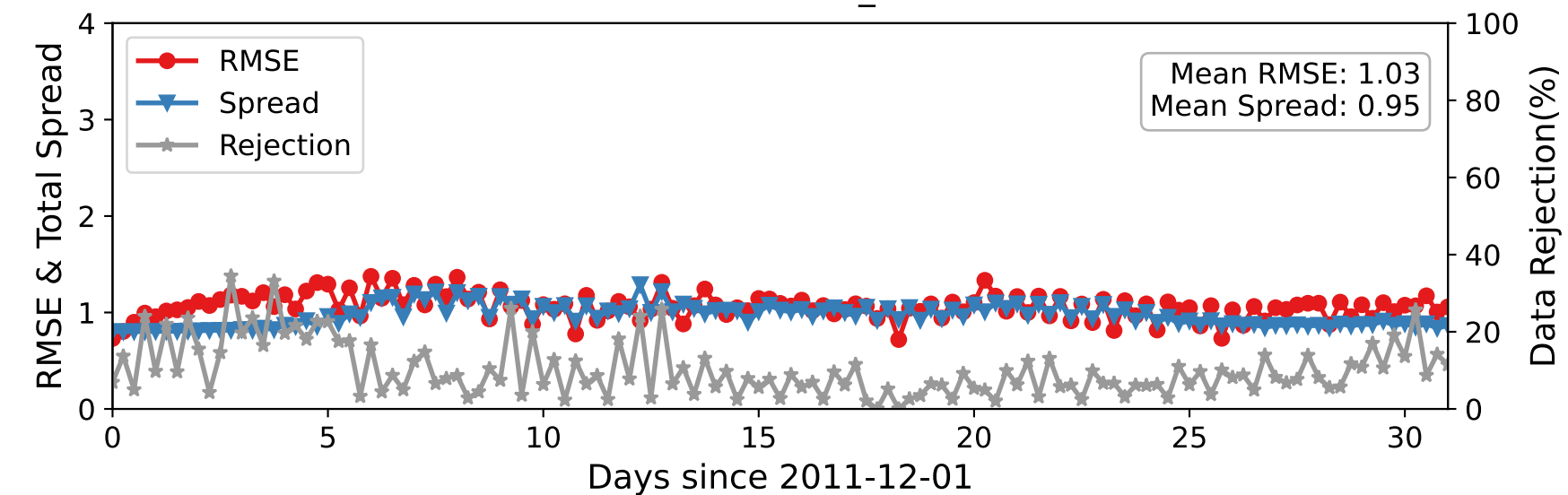
DARTEN20 — RADIOSONDE_T at 450-600 hPa
