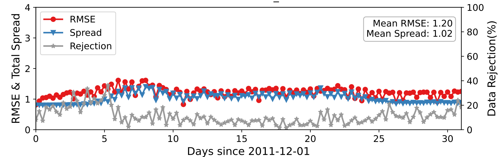
DARTEN20 — RADIOSONDE_T at 600-775 hPa
