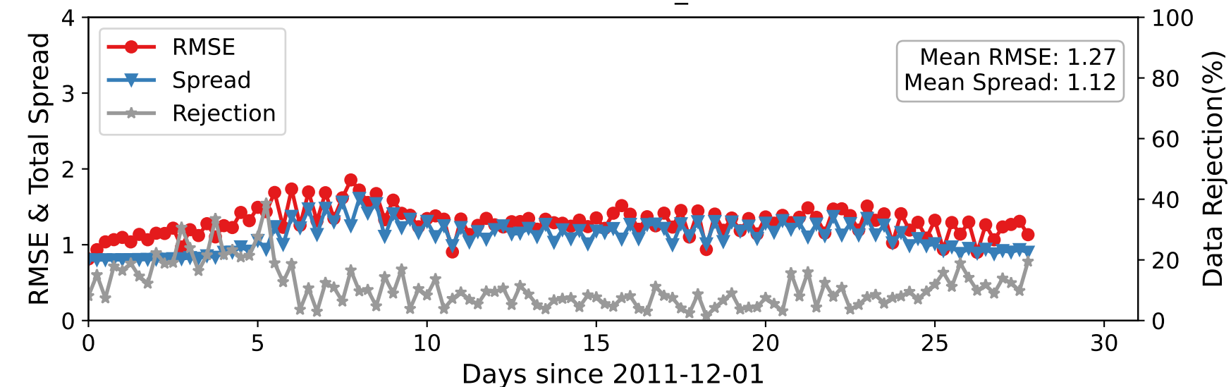
DARTEN10 — RADIOSONDE_T at 600-775 hPa
