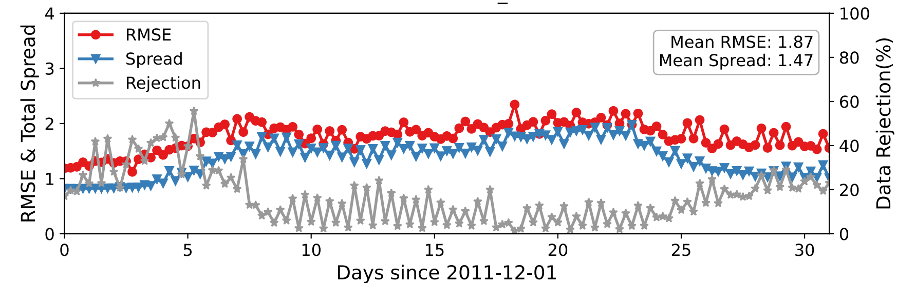
DARTEN20 — RADIOSONDE_T at 75-125 hPa
