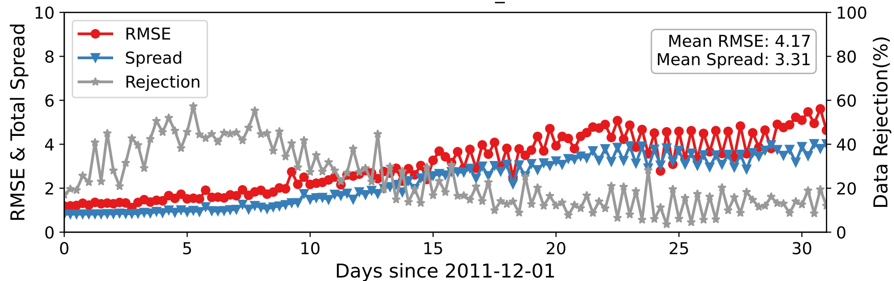
CTRLN10 — RADIOSONDE_T at 75-125 hPa
