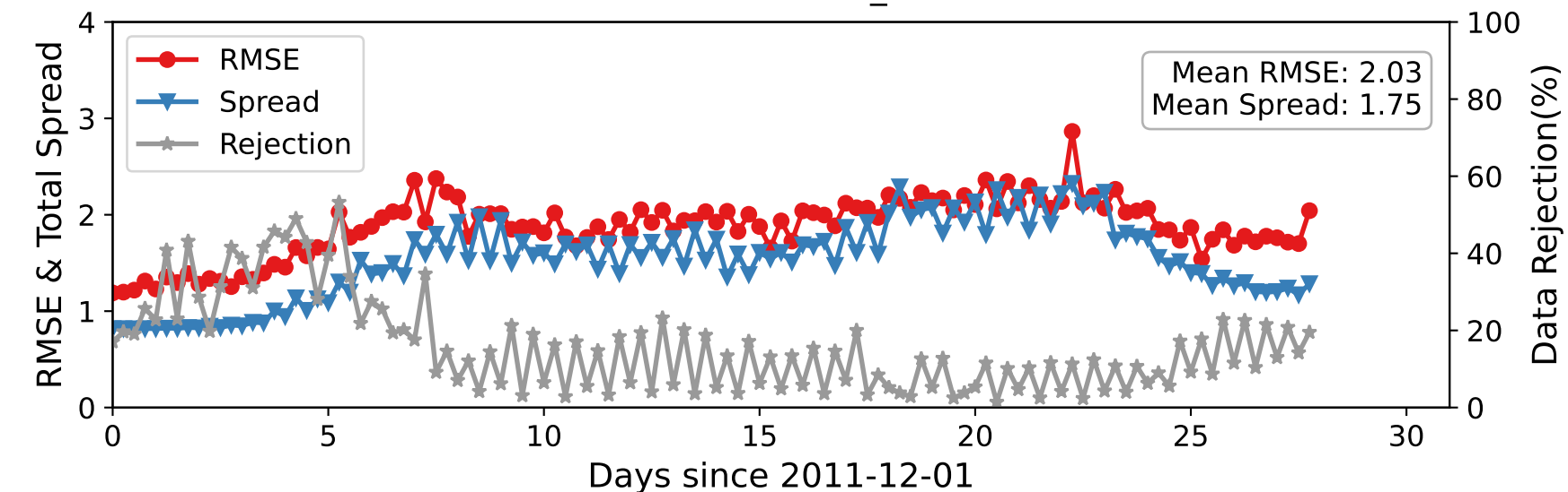
DARTEN10 — RADIOSONDE_T at 75-125 hPa
