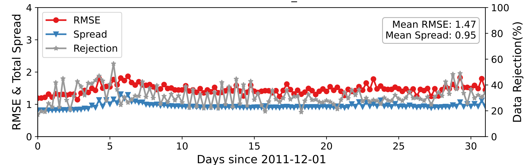
DARTEN40 — RADIOSONDE_T at 75-125 hPa
