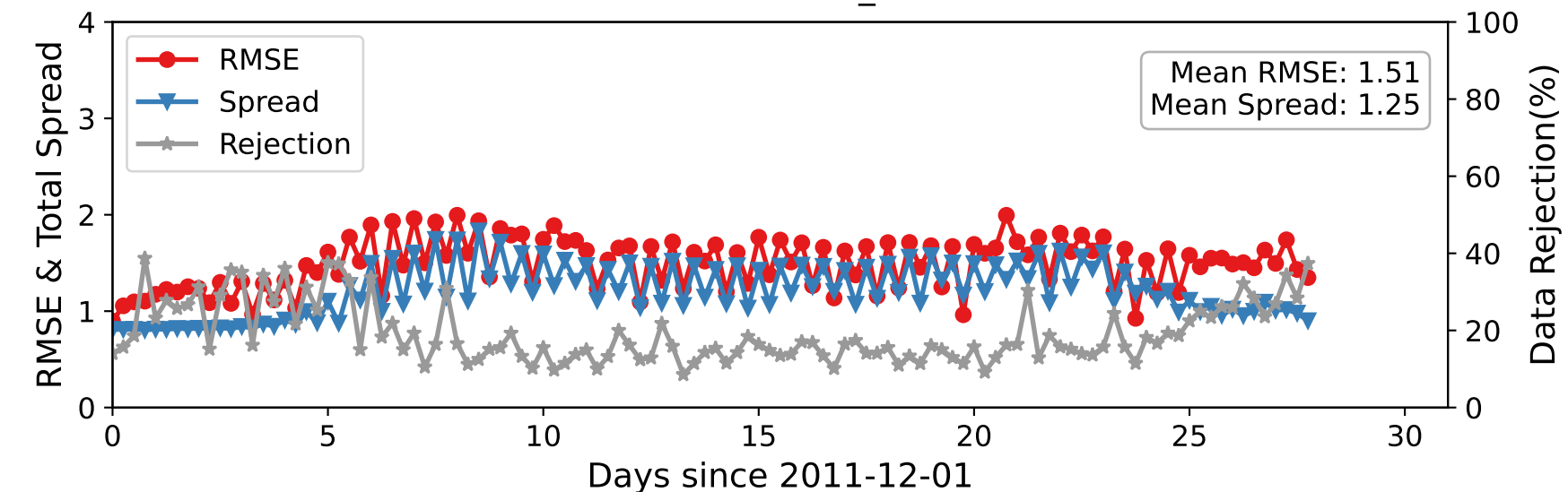
DARTEN10 — RADIOSONDE_T at 775-887 hPa
