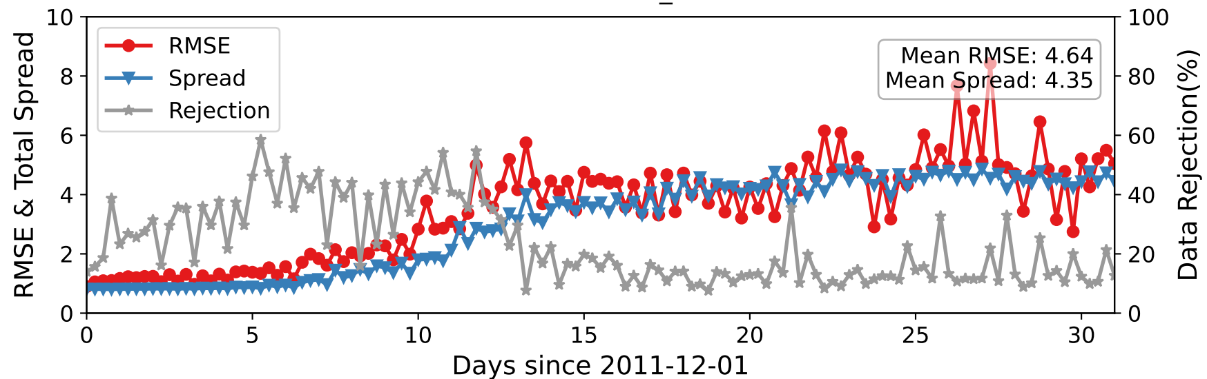
CTRLN10 — RADIOSONDE_T at 775-887 hPa
