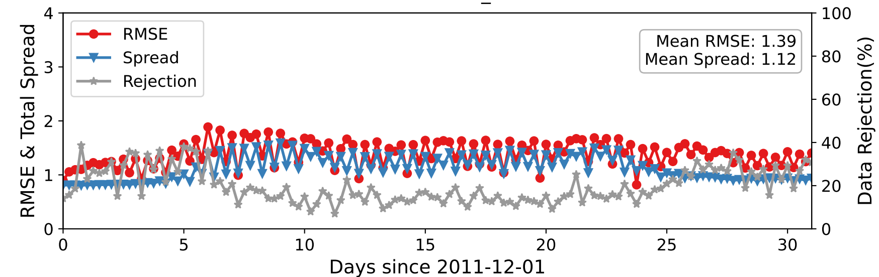
DARTEN20 — RADIOSONDE_T at 775-887 hPa
