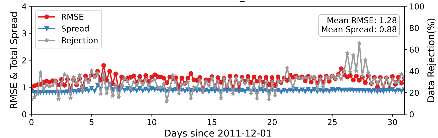
DARTEN40 — RADIOSONDE_T at 775-887 hPa
