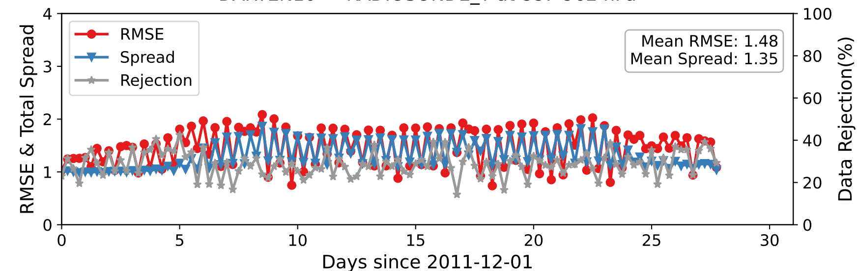
DARTEN10 — RADIOSONDE_T at 887-962 hPa
