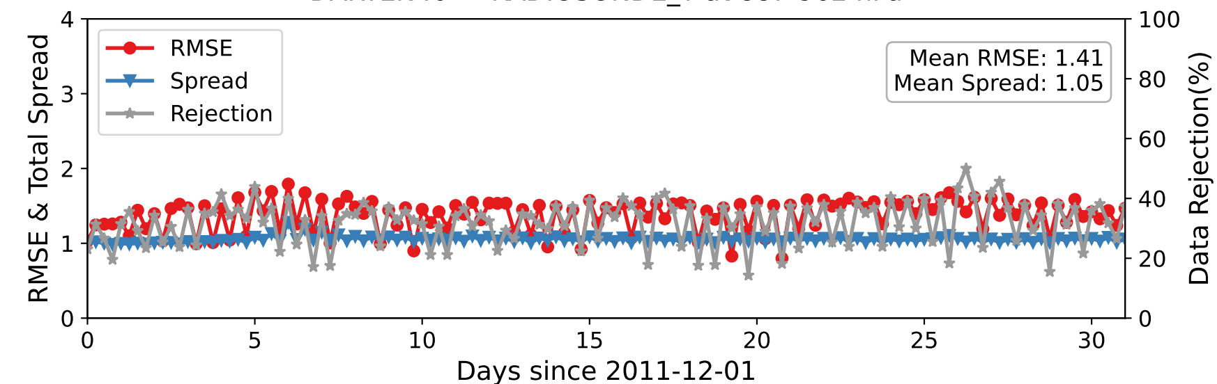
DARTEN40 — RADIOSONDE_T at 887-962 hPa
