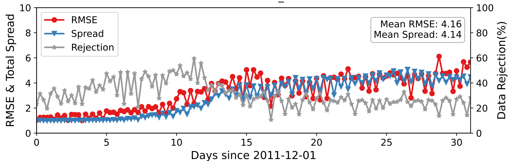
CTRLLEN10 — RADIOSONDE_T at 887-962 hPa
