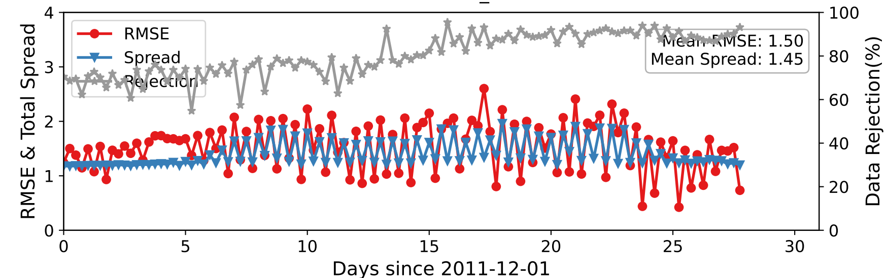
DARTEN10 — RADIOSONDE_T at 962-1035 hPa
