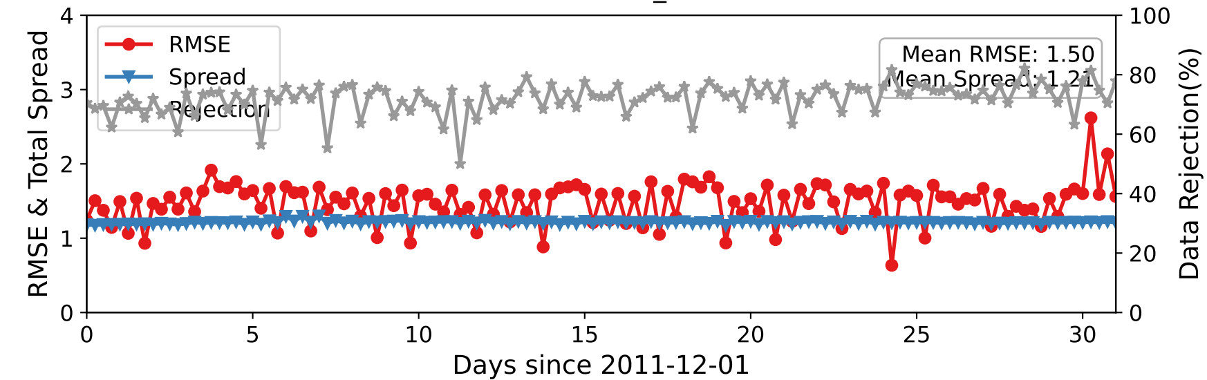
DARTEN40 — RADIOSONDE_T at 962-1035 hPa
