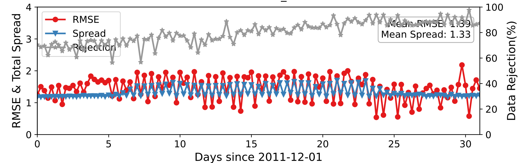
DARTEN20 — RADIOSONDE_T at 962-1035 hPa
