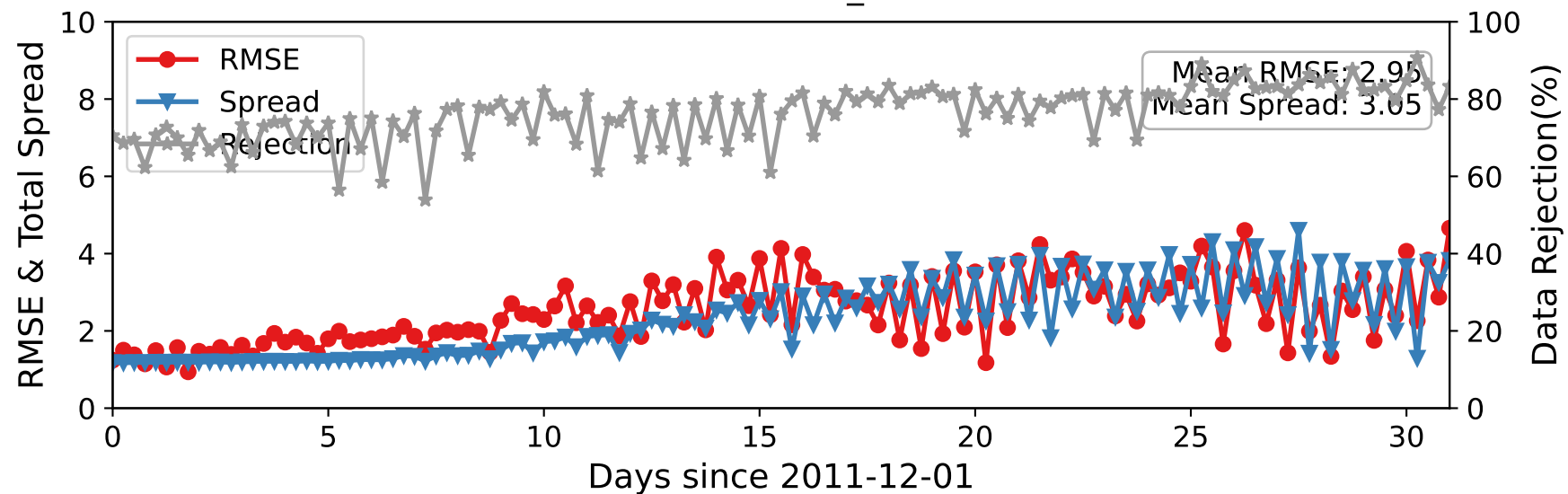
CTRLN10 — RADIOSONDE_T at 962-1035 hPa
