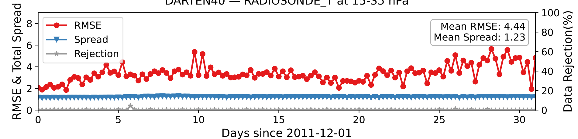
DARTEN40 — RADIOSONDE_T at 15-35 hPa
