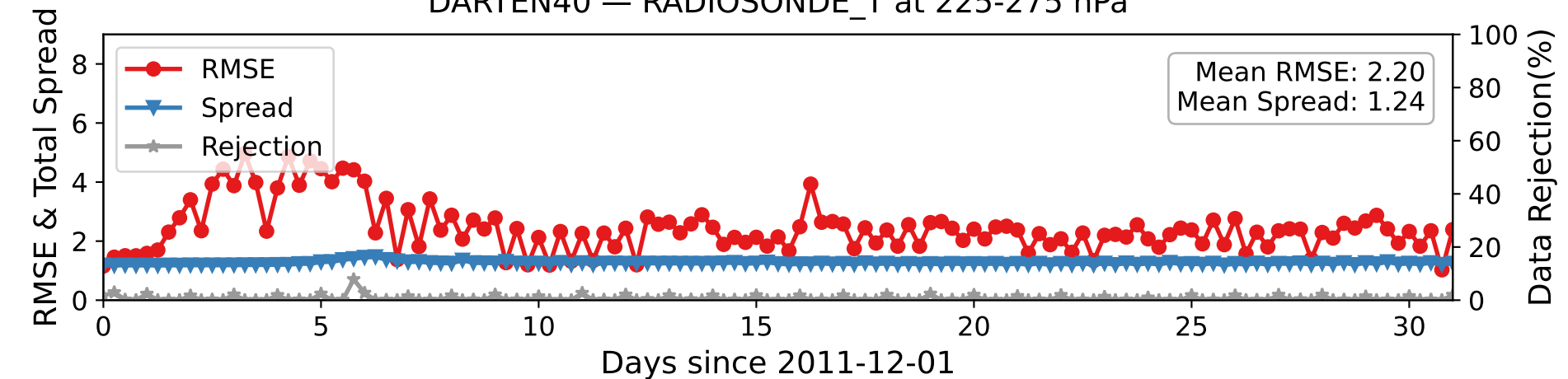
DARTEN40 — RADIOSONDE_T at 225-275 hPa
