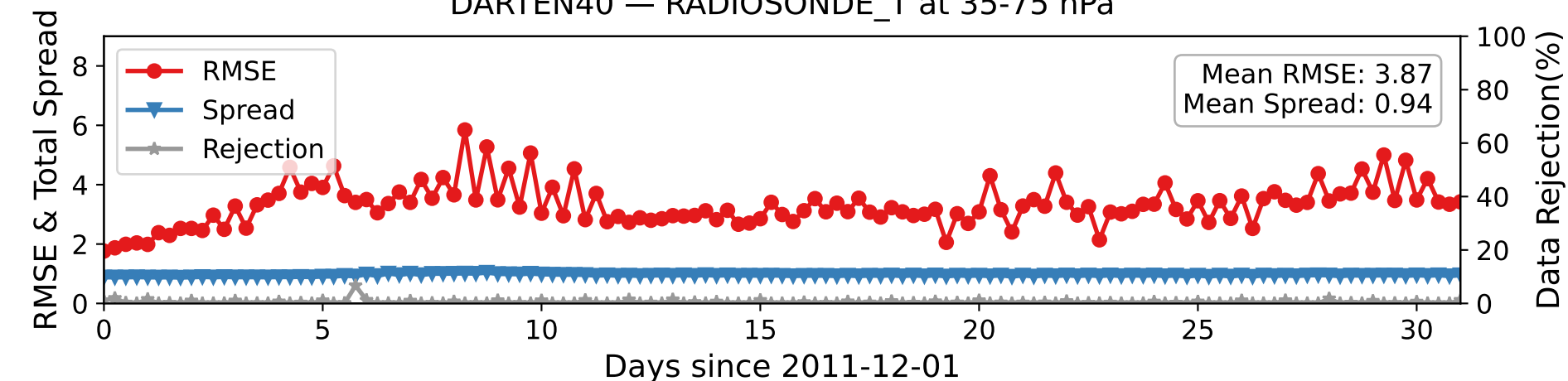
DARTEN40 — RADIOSONDE_T at 35-75 hPa
