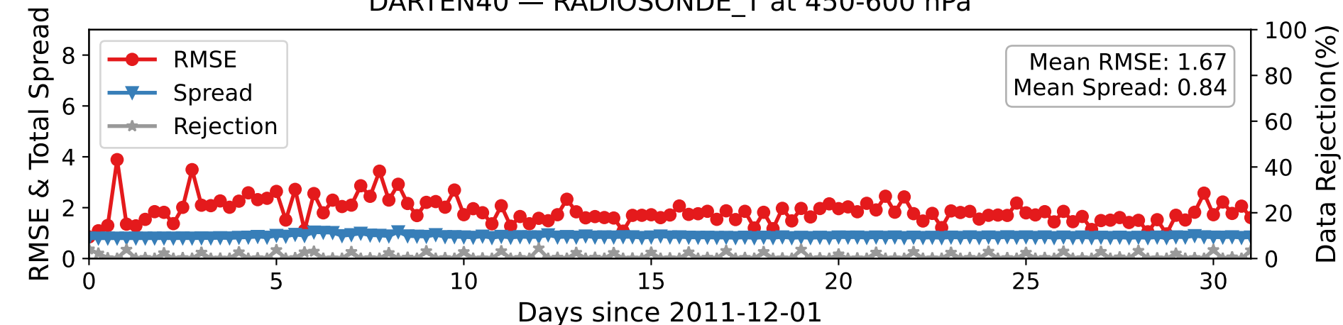
DARTEN40 — RADIOSONDE_T at 450-600 hPa
