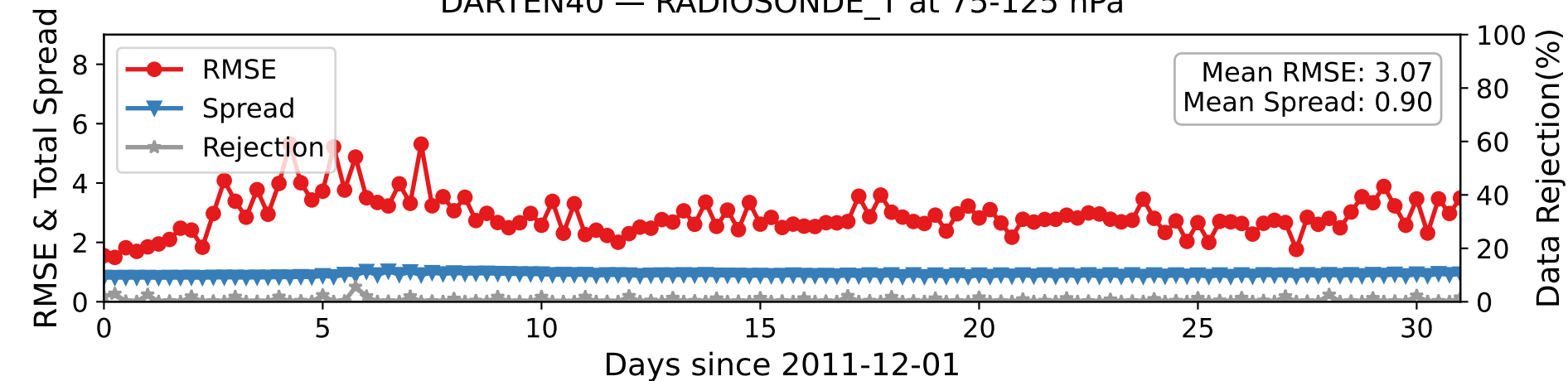
DARTEN40 — RADIOSONDE_T at 75-125 hPa
