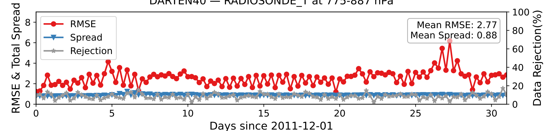
DARTEN40 — RADIOSONDE_T at 775-887 hPa
