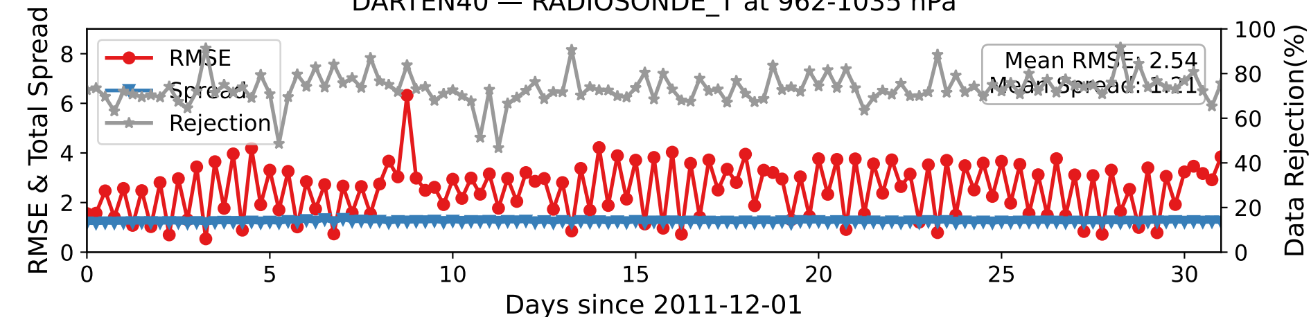
DARTEN40 — RADIOSONDE_T at 962-1035 hPa
