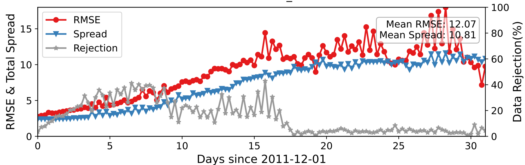
CTRLN10 — RADIOSONDE_U at 125-175 hPa
