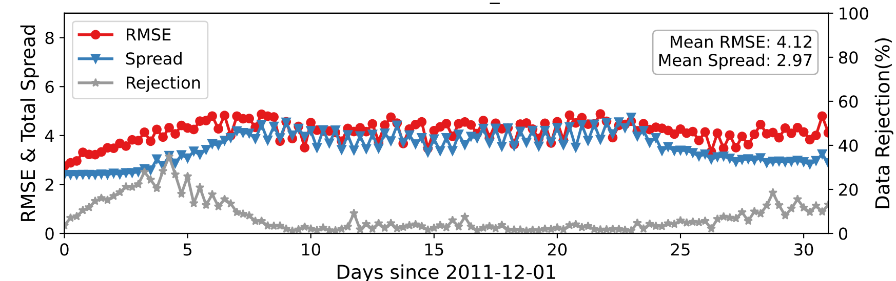
DARTEN20 — RADIOSONDE_U at 125-175 hPa
