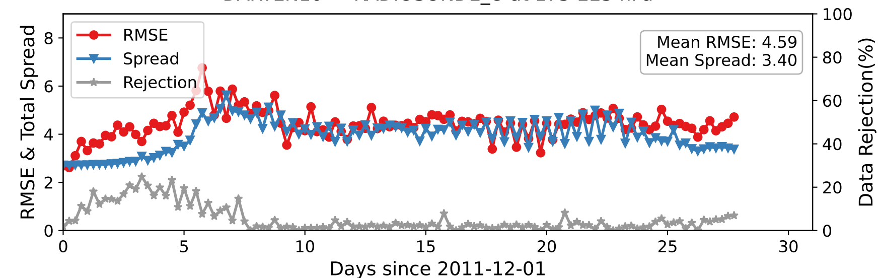
DARTEN10 — RADIOSONDE_U at 175-225 hPa
