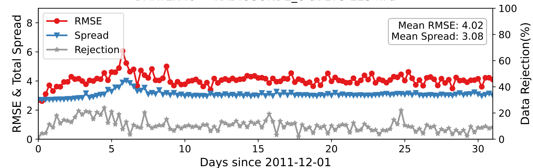
DARTEN40 — RADIOSONDE_U at 175-225 hPa
