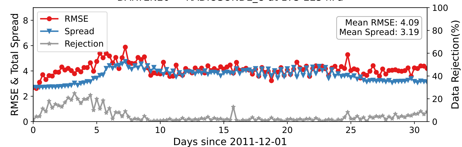
DARTEN20 — RADIOSONDE_U at 175-225 hPa
