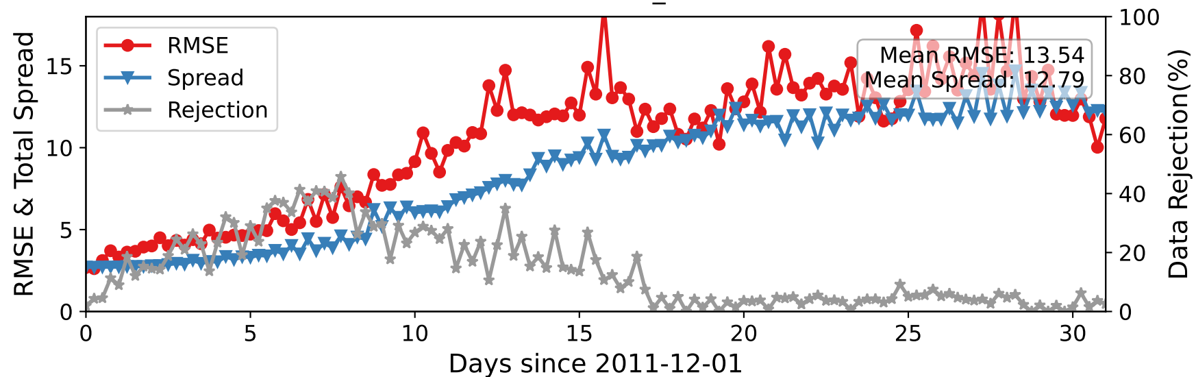
CTRLN10 — RADIOSONDE_U at 175-225 hPa
