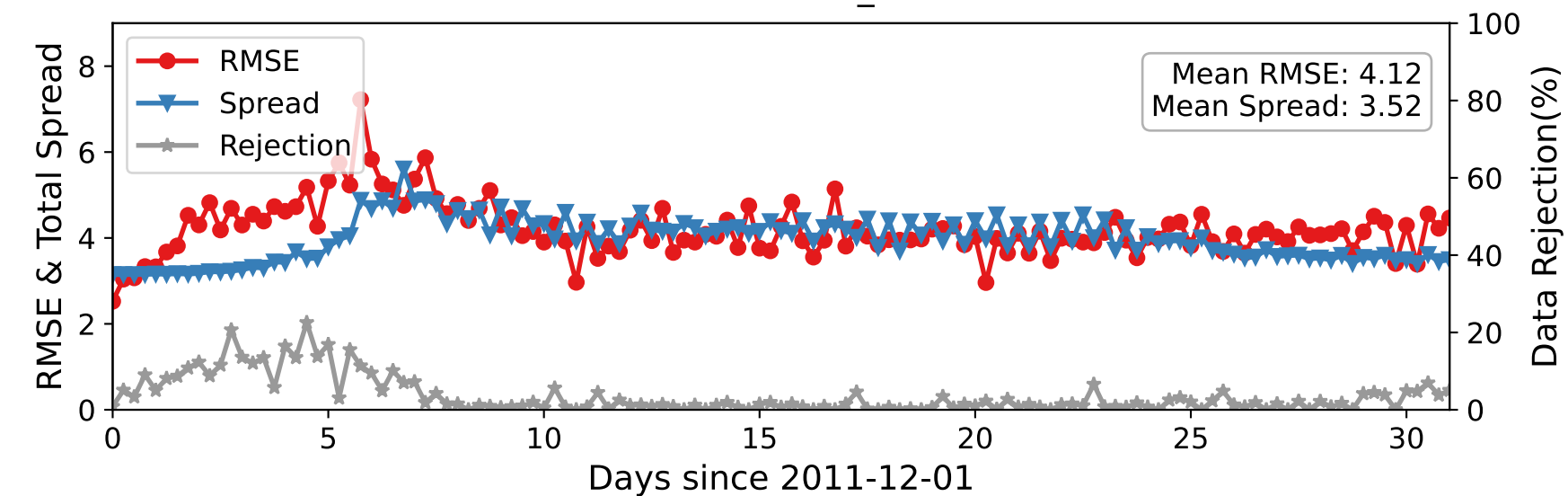
DARTEN20 — RADIOSONDE_U at 225-275 hPa
