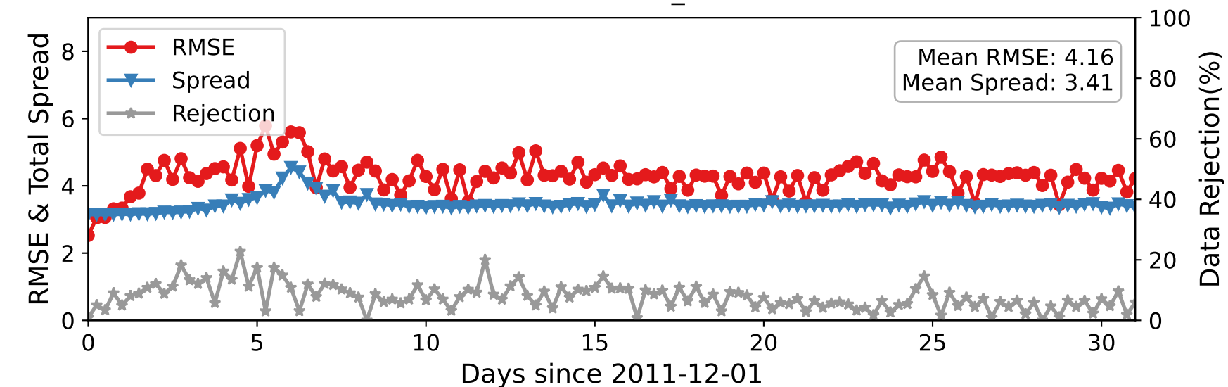
DARTEN40 — RADIOSONDE_U at 225-275 hPa
