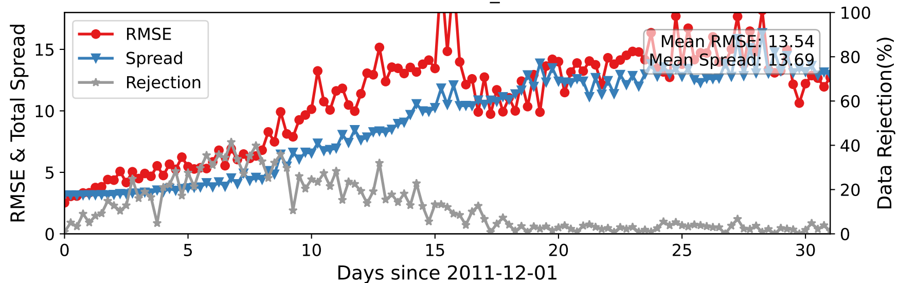
CTRLN10 — RADIOSONDE_U at 225-275 hPa
