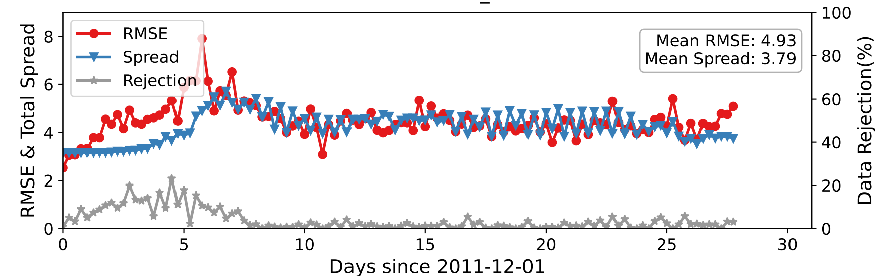
DARTEN10 — RADIOSONDE_U at 225-275 hPa
