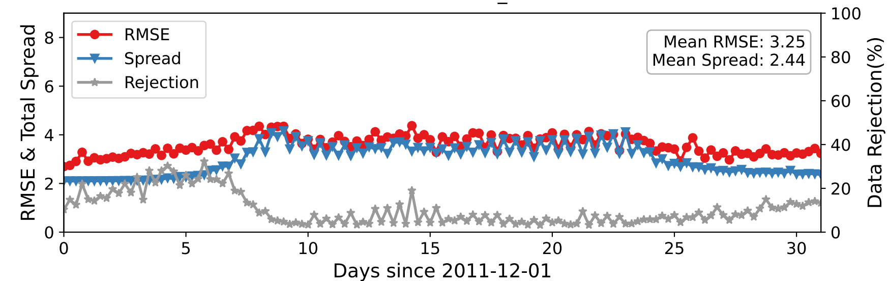
DARTEN20 — RADIOSONDE_U at 35-75 hPa
