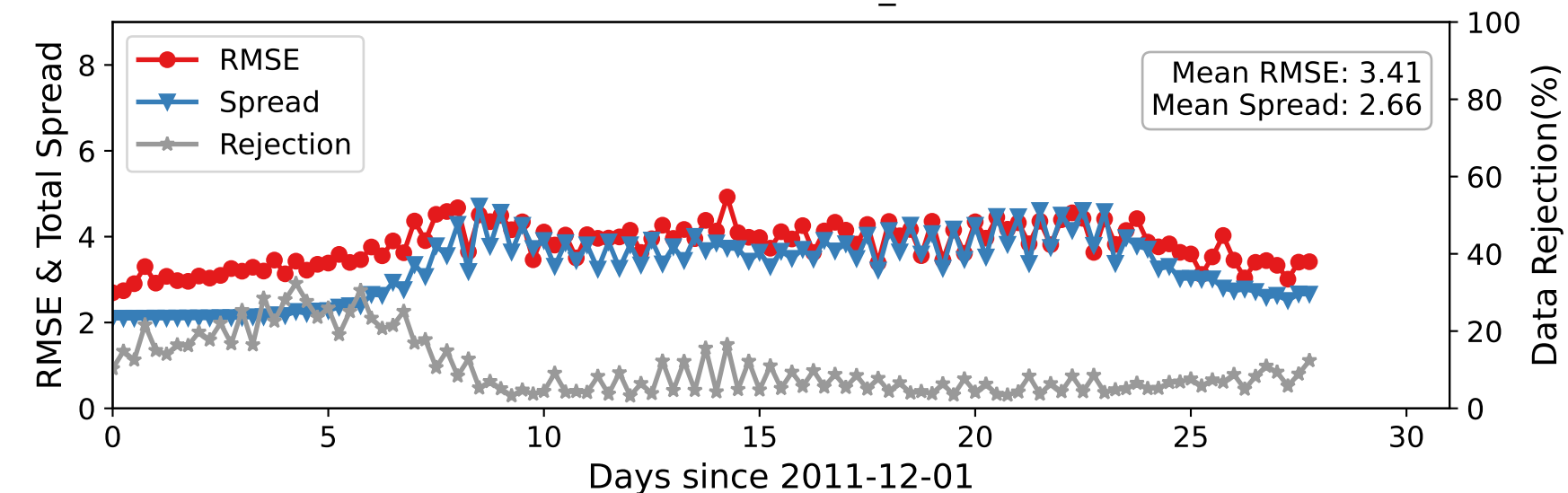
DARTEN10 — RADIOSONDE_U at 35-75 hPa
