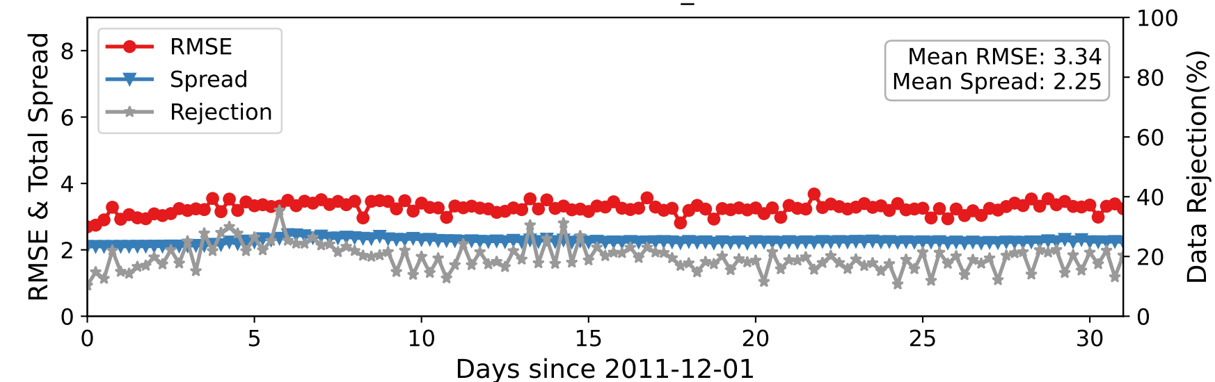
DARTEN40 — RADIOSONDE_U at 35-75 hPa
