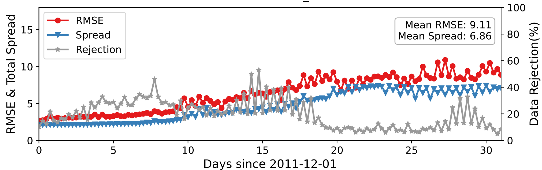
CTRLN10 — RADIOSONDE_U at 35-75 hPa
